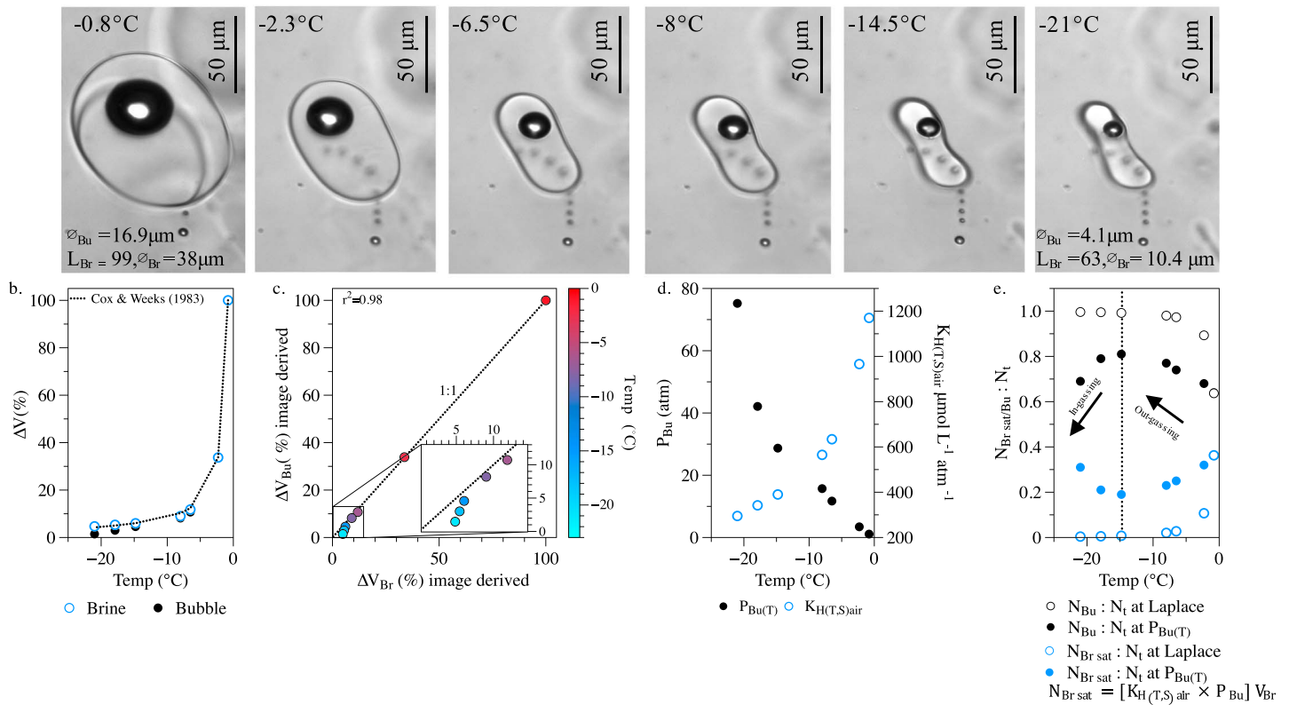
Figure 3. (a) Microphotographs of cooling experiment 1 clearly show decreases in discrete brine pocket size with decreasing temperature and simultaneous decrease in size of a bubble contained therein. (b) Relative volume change \Delta V (in %) from initial stage of both the discrete brine pocket and its contained bubble with decreasing temperature computed from the images presented in (a). (c) Relative changes in bubble volume versus relative changes in brine volume (dotted line is the 1:1 relationship). (d) Bubble inner pressure ( P_{Bu(T)} ) and Henry's constant ( K_{H(T,S)air} ) with decreasing temperature. (e) The number of moles of gas dissolved in brine ( N_{Br sat} : N_t ) and in the air bubble ( N_{Bu} : N_t ) as a fraction of the total number of moles in the closed brine + bubble system with decreasing temperature (see text for details of computation).
