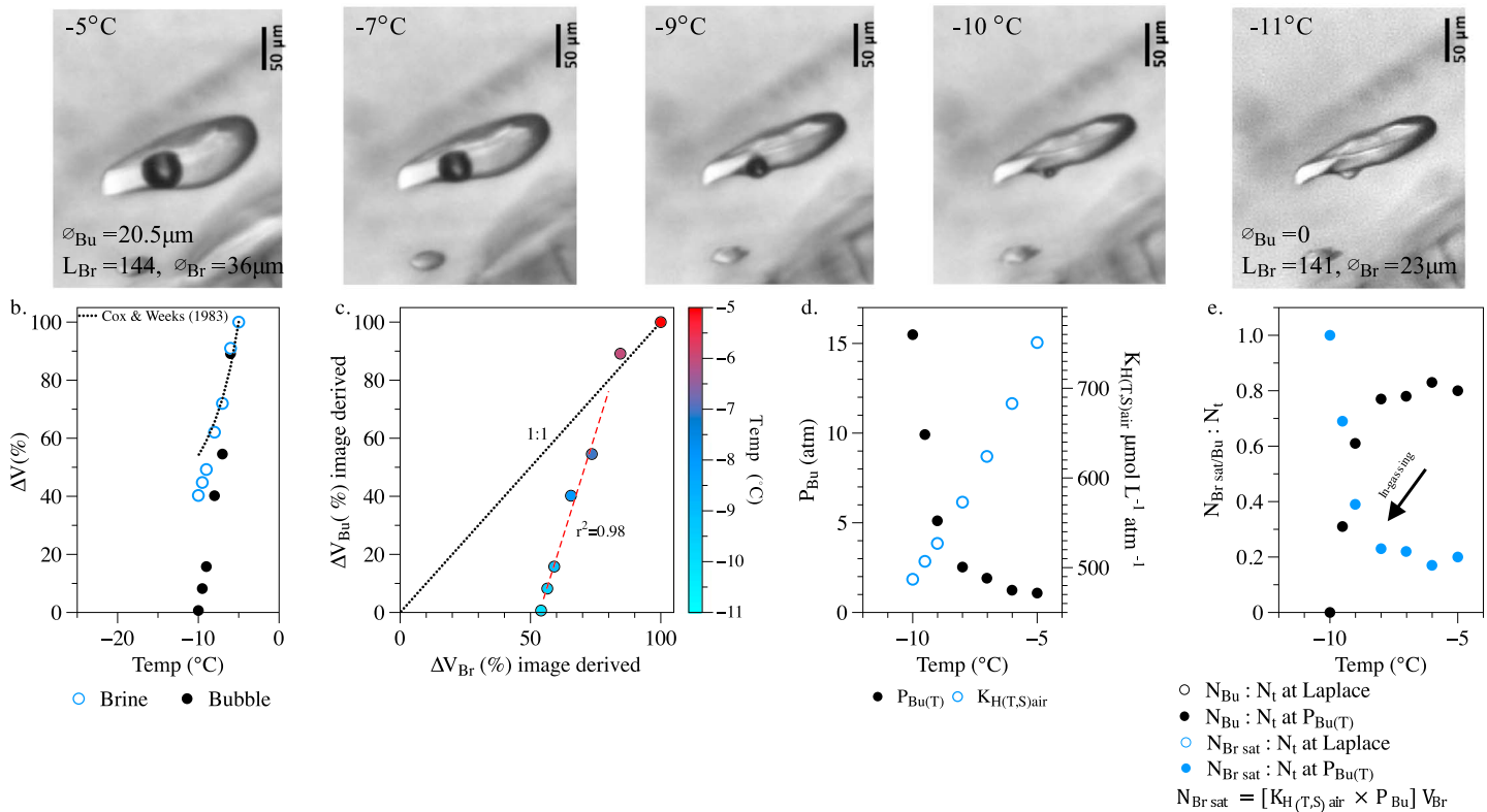
Figure 4. (a) Microphotographs of cooling experiment 2 clearly show decreases in discrete brine pocket size with decreasing temperature and simultaneous decrease in size of a bubble contained therein, which eventually disappears. (b) Relative volume change \Delta V (in %) from initial stage of both the discrete brine pocket and its contained bubble with decreasing temperature computed from the images presented in (a). (c) Relative changes in bubble volume versus relative changes in brine volume, (dotted line is the 1:1 relationship, the red line is fitted line using linear regression). (d) Bubble inner pressure ( P_{Bu(T)} ) and Henry's constant ( K_{H(T,S)air} ) with decreasing temperature. (e) The number of moles of gas dissolved in brine ( N_{Br sat} : N_t ) and in air bubble ( N_{Bu} : N_t ) as a fraction of the total number of moles in the closed brine + bubble system with decreasing temperature.
