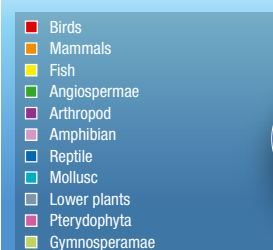
Figure 7: Species groups targeted by LIFE projects (1992-2008)
