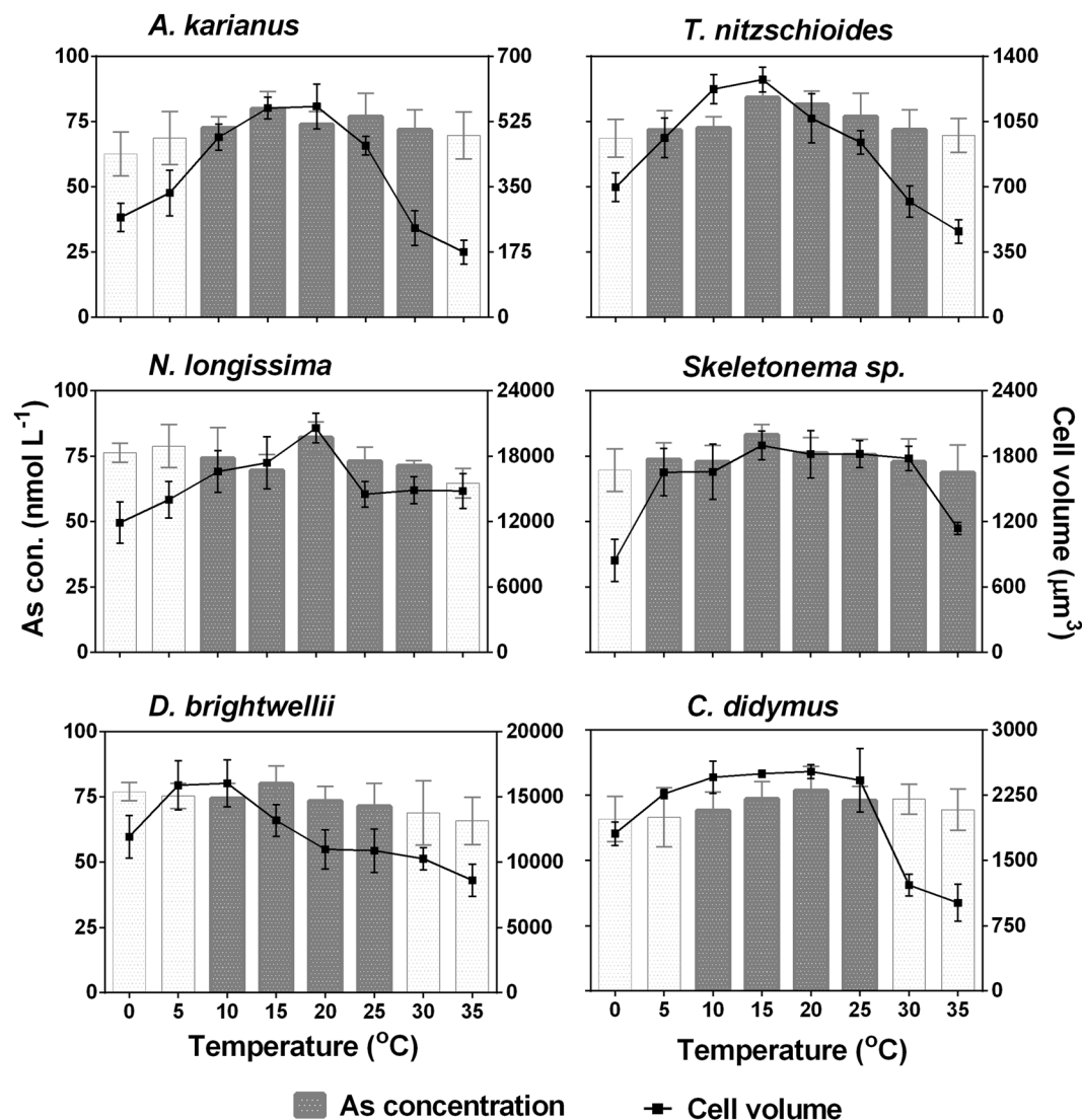
Figure 8. Relationship between cell size and As biotransformation of six marine diatom species at various temperature levels. Dark bars in the graph indicate As species biotransformation occurred, i.e. As(V) was reduced to As(III) and the subsequent methylation to MMAA and DMAA. White bars indicate no biotransformation occurred, i.e. only As(V) was detected in the culture medium. Data are means ± SD (n = 3).
