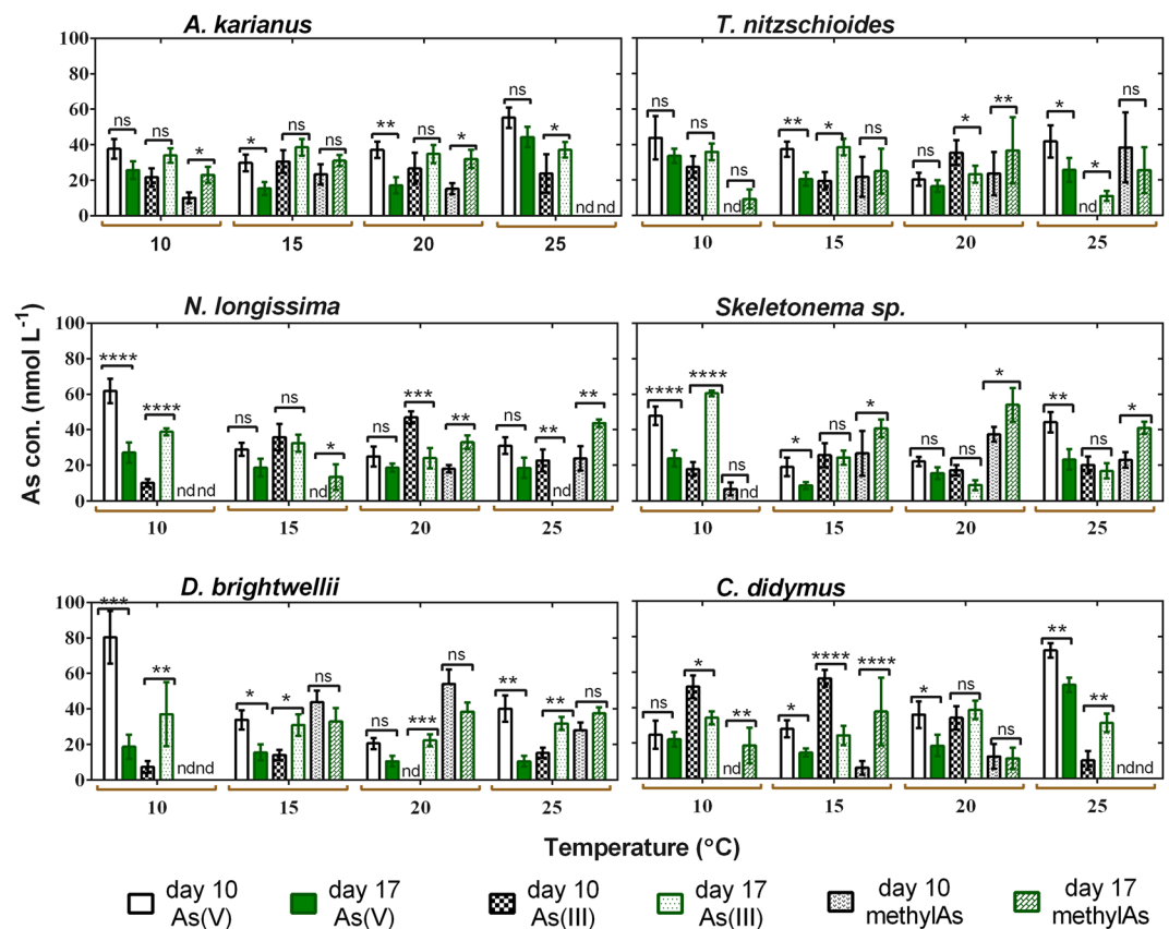
Figure 6. Time-dependent As speciation patterns by six marine diatom species. As speciation was observed on day 10 and 17 of culture at various temperatures (°C). The star marks above the bars showed significant differences at *p \leq 0.01 , **p \leq 0.001 , and ***p \leq 0.0001 levels between day 10 and 17 within the same As species. 'ns' indicates non-significant, 'nd' indicates not detected. Data are means \pm SD ( n = 3 ).
