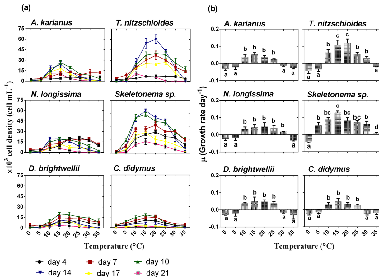
Figure 2. Effect of temperature (°C) on the growth of marine diatom species, (a) cell density (cell mL -1 ), (b) growth rate day -1 . Different lowercase letter in Fig. 2(b) indicates significant differences between temperature levels. Data are means ± SD ( n = 3).
