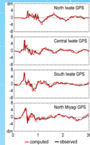
Computed sea surface elevations show excellent agreement with the observed GPS buoy data (Y. Yamazaki and K.F. Cheung, Univ. of Hawaii).
