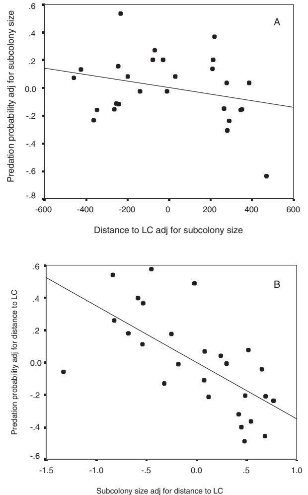
FIG. 3. – (A) Relationship between the probability of predation and distance to nearest sub-colony of yellow-legged gulls adjusted for sub-colony size (Partial correlation, r = -0.282, n = 27, d.f. = 24, p = 0.163 ). (B) Relationship between the probability of predation and sub-colony size adjusted for distance to nearest sub-colony of yellow-legged gulls (Partial correlation, r = -0.668, n = 27, d.f. = 24, p < 0.001 ).
