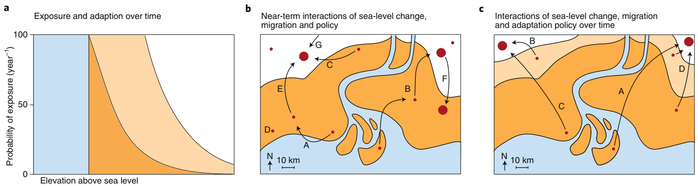
Fig. 1 | Migration under sea-level change and policy scenarios. a , A framework for evaluating risk of exposure occurring by the year 2050, when global mean sea-level rise is similar under different emission scenarios, based on the likelihood of hazards related to sea-level change occurring in any given area during a given year. Mean sea level is indicated by the border between blue and orange regions. b , Exposure and migration dynamics that may emerge simultaneously in this period, their various triggering mechanisms and potential policies that may act as intervening factors. Migration is depicted (arrows) between potential destinations (red circles, the size of which correspond to rising and falling rates of migration). In the short term, policy may simultaneously influence various forms of mobility and migration at sea level including (A) short-distance, temporary or seasonal migration, (B) urbanization in coastal cities, (C) permanent migration from rural areas, (D) mobility traps, (E) prospective migration in advance of impacts, (F) short-term ‘climate gentrification’ of high-risk areas and (G) background pro-coastal migration. c , The possibility space for one projection of sea-level change under an unspecified emission scenario at the year 2100, with associated adaptation interventions and migration outcomes. Areas in flood plains will be inundated with increasing frequency (dark orange), and new areas formerly above the annual flood plain will experience intensifying risk (orange). Adaptation interventions will increasingly affect migration dynamics, including (A) the concentration of multiple migration flows to fewer safe destinations where coastal fortification and accommodation has occurred, (B) settlement abandonment where no adaptation interventions have occurred, (C) community relocation accompanying a strategy of retreat and (D) sudden migration as adaptation interventions reach their limits.
