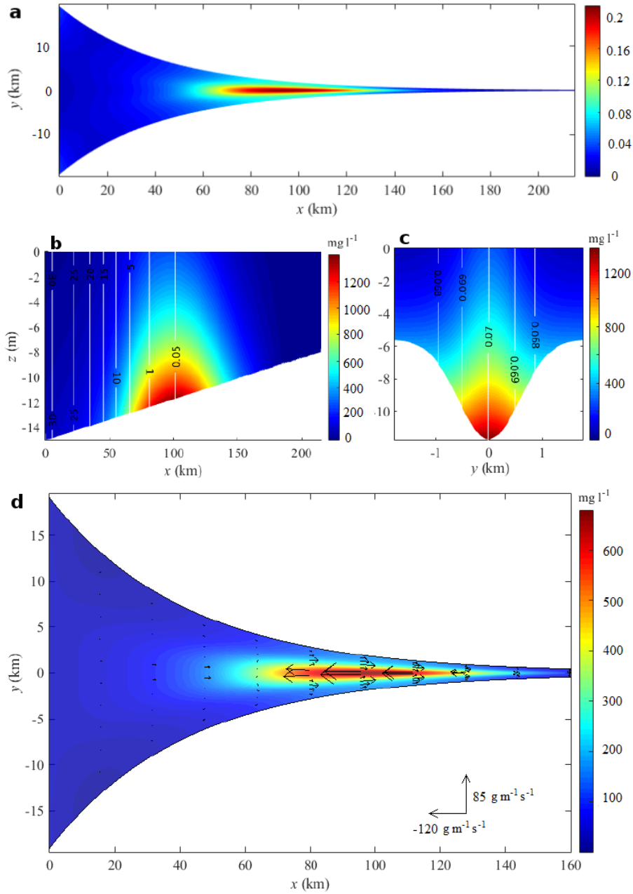
Figure 4.11: The same as Fig. 4.8, but for w_s = 1 \text{ mm s}^{-1} and d_s = 40 \text{ }\mu\text{m} . The cross-section in Fig. 4.11c is taken at x = 100 \text{ km} .
