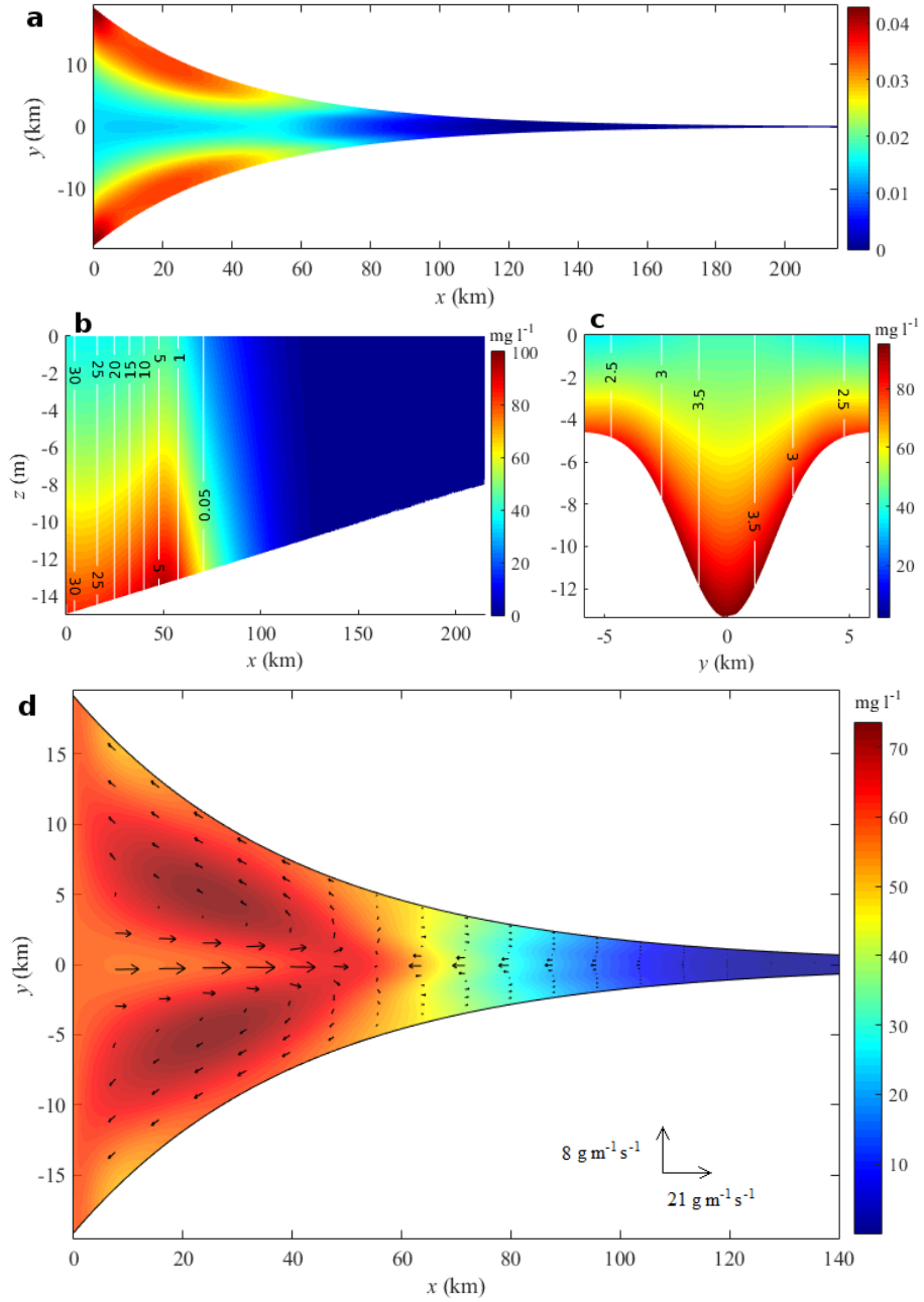
Figure 4.15: The same as Fig. 4.8, but for R = 864 \text{ m}^3 \text{ s}^{-1} . The cross-section in Fig. 4.15c is taken at x = 50 \text{ km} .
