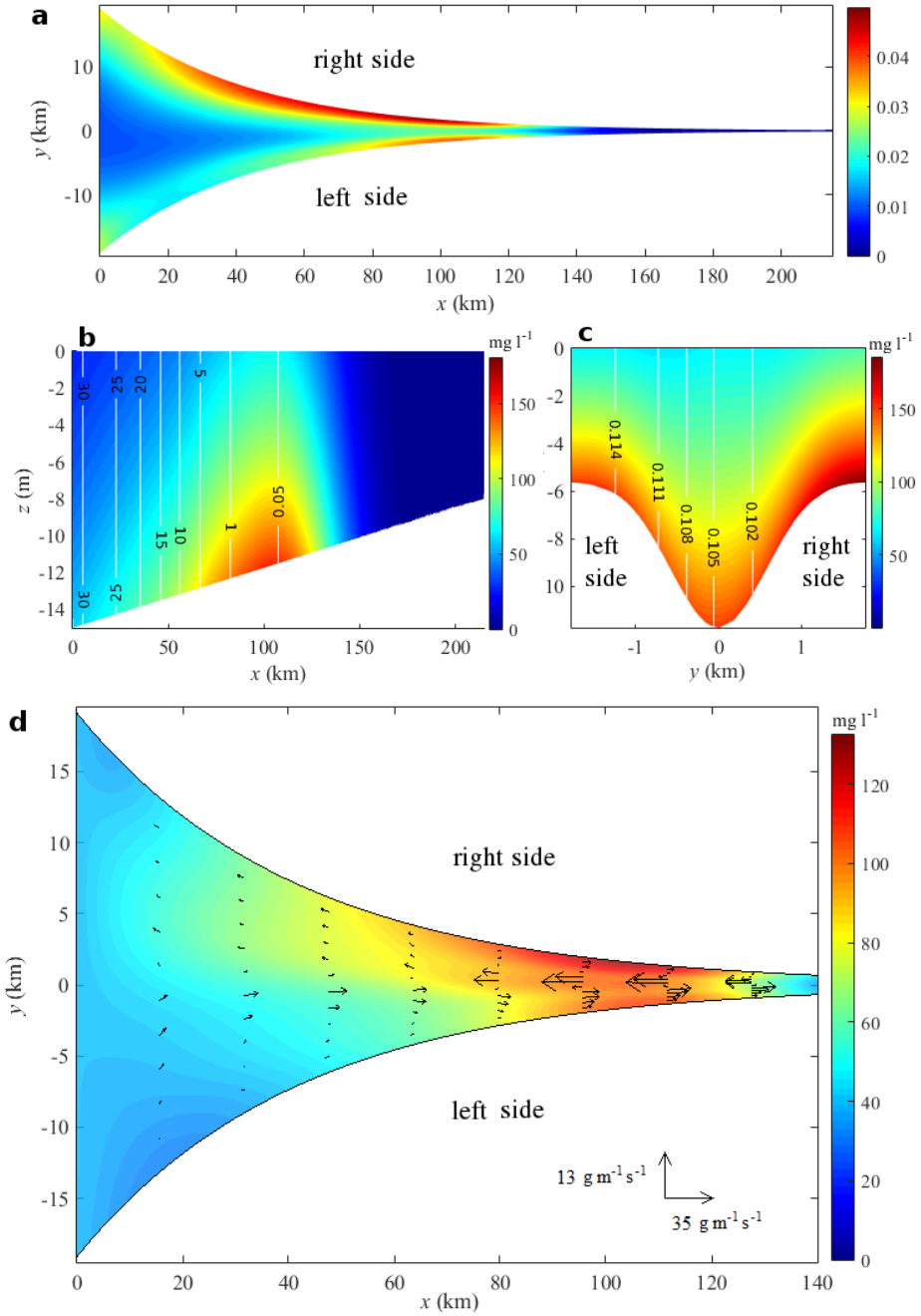
Figure 4.8: The same as Fig. 4.3 and Fig. 4.4, but for f = 1 \times 10^{-4} \text{ rad s}^{-1} .
