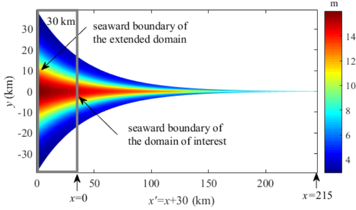
Figure 4.2: The bathymetry and geometry of the extended domain, and the (non-extended) domain of interest.
