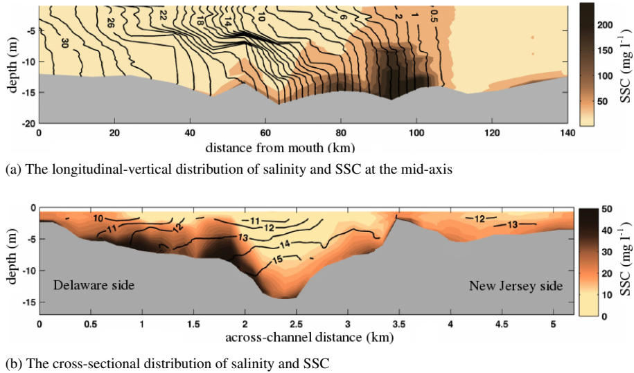
Figure 1.4: The observed distributions of salinity and sediment concentration in the Delaware estuary. The figures are based on McSweeney et al. (2016), and reprinted with permission.
