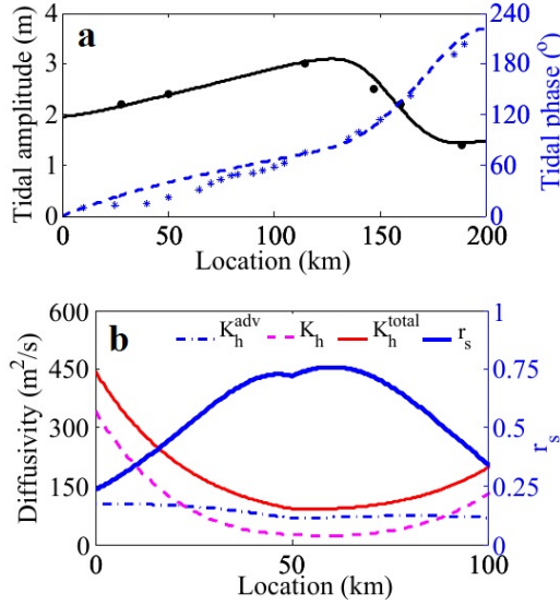
Figure 2.9: (a) The modelled M_2 sea surface amplitude (see black solid line) and phase (blue dashed line) versus the observed M_2 tidal surface amplitude (black dots) and phase (blue stars) in the Scheldt estuary. (b) Diffusivity ( K_h^{adv} , K_h , and K_h^{total} ) and the ratio r_s in the region of salt intrusion.
