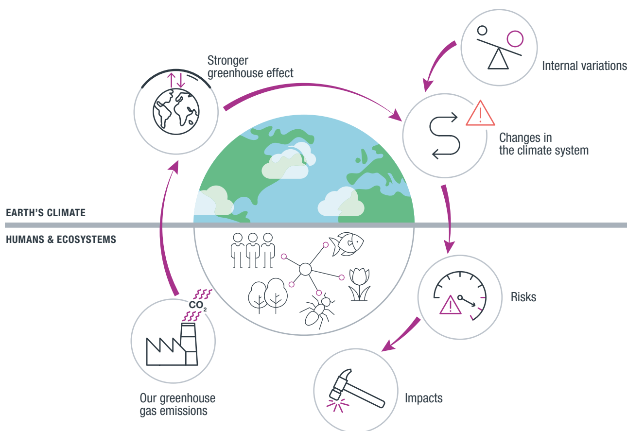
Flow diagram of human greenhouse gas emissions and the impacts of climate change
