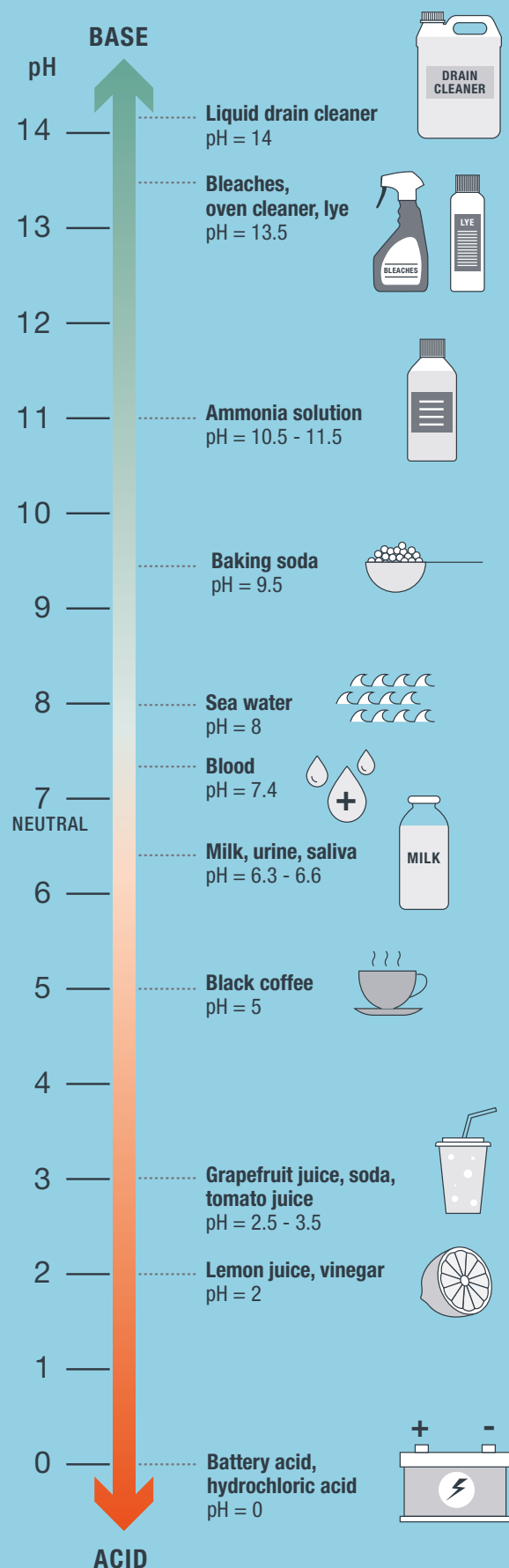
pH scale and examples of different solutions.
