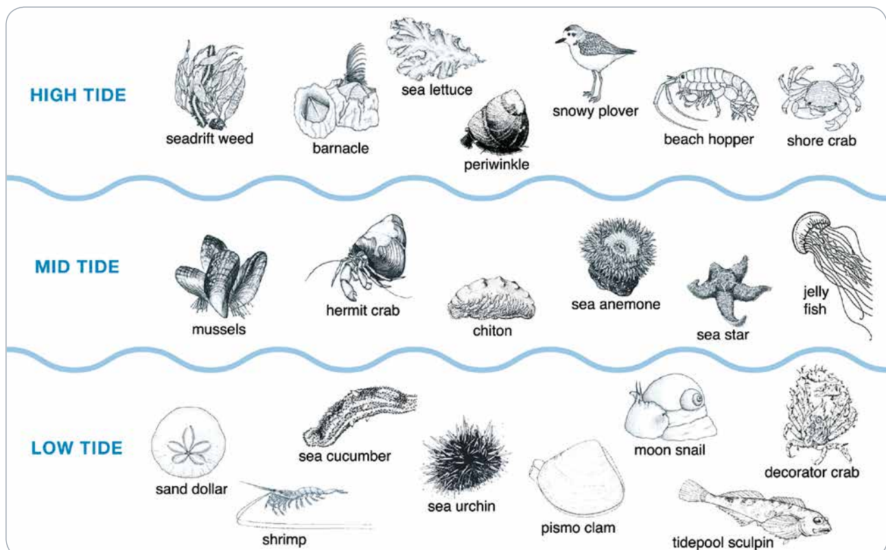
Common plants and animals found between the high and low water mark (illustration compiled by Aurèle Clemencin).
