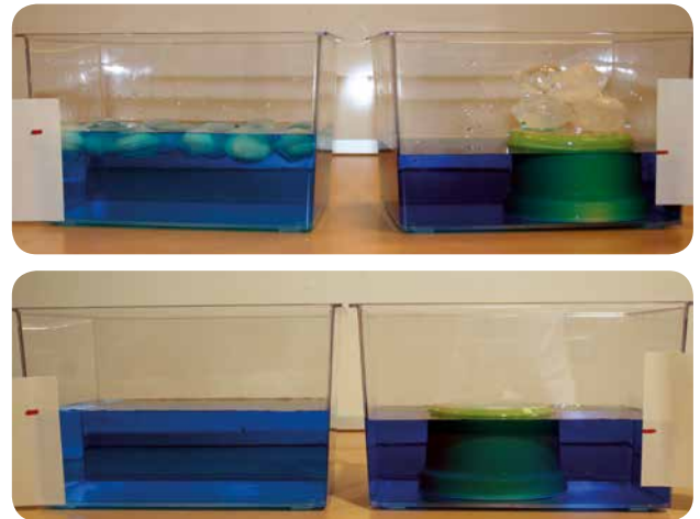
Top: before ice melting. Bottom: after ice melting.
