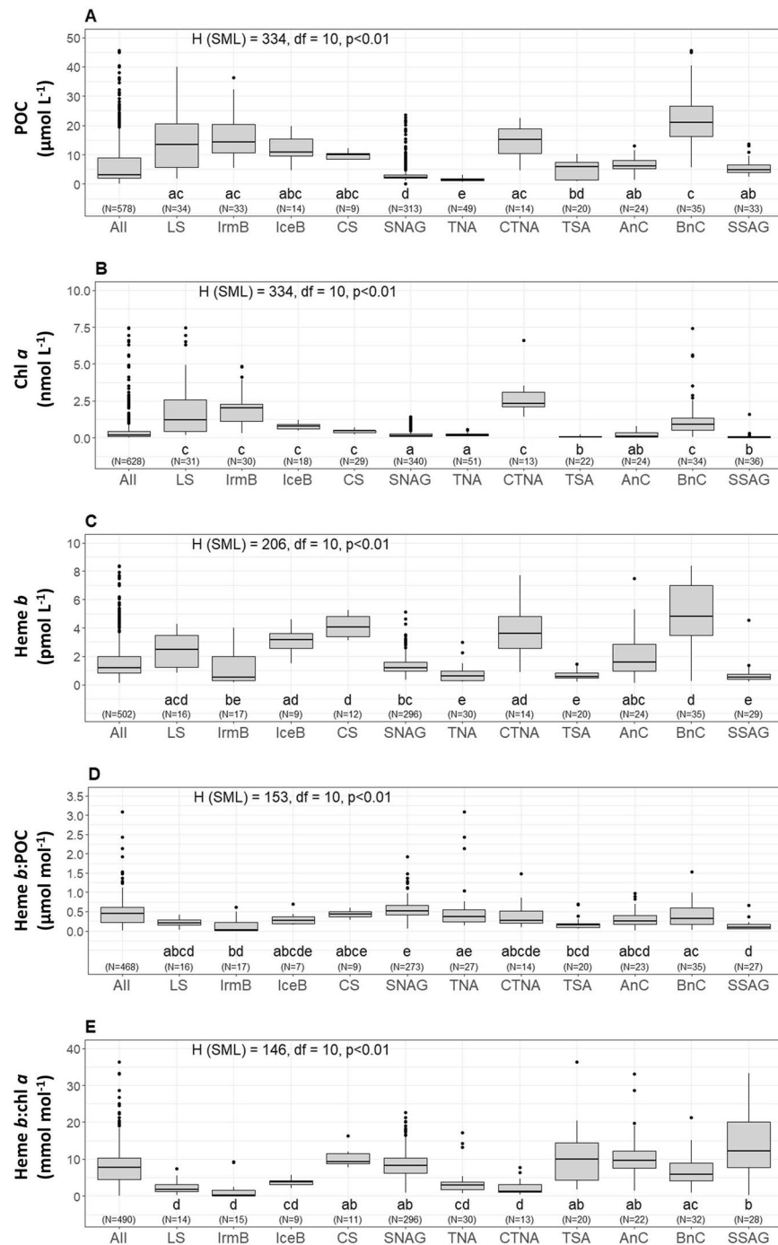
Figure 3. Boxplots of distributions in the surface mixed layer (SML) of (A) Particulate Organic Carbon (POC), (B) chlorophyll a (chl a ), (C) heme b , (D) the ratio heme b :POC, and (E) the ratio heme b :chl a for the eleven oceanographic regions; Labrador Sea (LS), Labrador Sea (LS), Irminger Basin (IrmB), Iceland Basin (IceB), Celtic Sea (CS), Subtropical North Atlantic Gyre (SNAG), Tropical North Atlantic (TNA), Coastal Tropical North Atlantic (CTNA), Tropical South Atlantic (TSA), Angola Current (AnC), Benguela Current (BnC) and Subtropical South Atlantic Gyre (SSAG). The boxes show the interquartile range (IQR) of values. The bold lines inside the boxes indicate the median value for each region and divide the boxes the 25th (bottom) and 75th (upper) percentiles. The upper whisker represents the largest value no farther than 1.5 times the IQR, and the bottom whisker indicates the smallest value no farther than 1.5 times the IQR. Dots represent the outliers of the distributions. On top of sub-plots A, B, C, D and E the result of the Kruskal–Wallis test is annotated. Letters (letters a to d) below the boxes indicate the Compact Letter Display (cld) of the statistically significant different groups in the SML after a Post-hoc test for multiple comparisons of groups. The numbers in brackets indicate the number of data points used per box for each parameter. The figure was produced using R Statistical Software 97 v.1.0.136 (R core team, 2016, https://www.R-project.org ).
