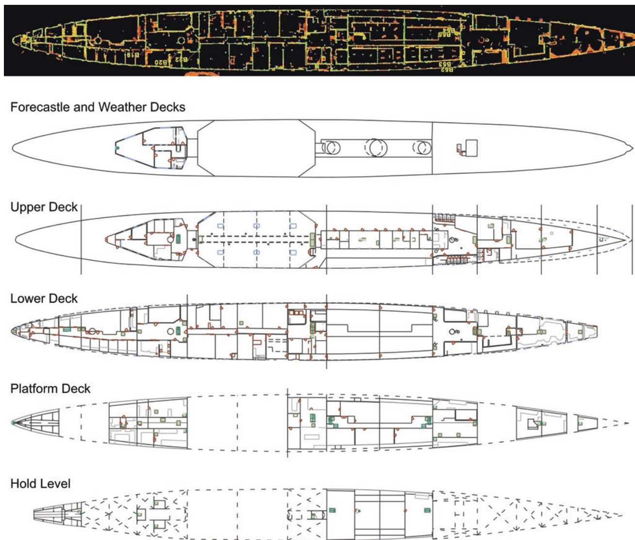
Fig. 7.10 2D output of the lower deck of HMS Caroline derived from the laser scan data (top) as indicated in a traditional plan (bottom). This allowed the most current representation of the compartments and spaces
