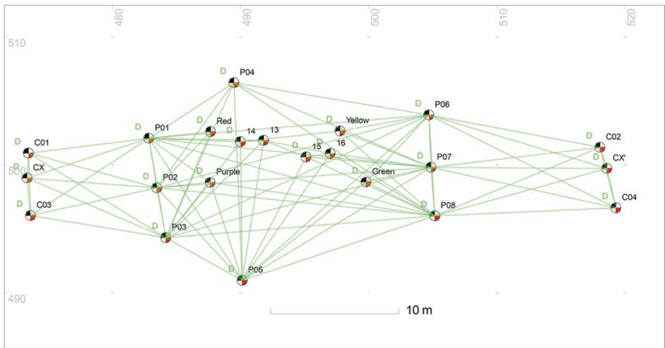
Fig. 4.5 Control points network, 2013 Gnalić Research Campaign (J.L. Casabán)
