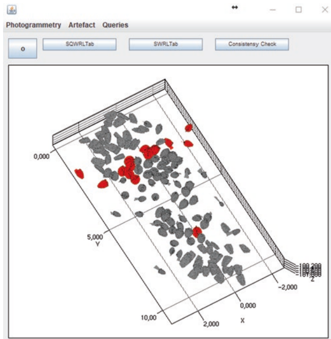
Fig. 9.1 3D visualization of a spatial resquest in SWRL: Amphorae(?a) \wedge swrlArp:isCloseTo(?a, "IdTargetAmphora", 6.2) \wedge hasTypologyName(?a, "Pitecusse\_365") \rightarrow sqwrl:select(?a) . Means select all amphorae with the typology Pitecusse_365 and at a maximum distance of 6.2 m from the amphorae labelled IdTargetAmphora
