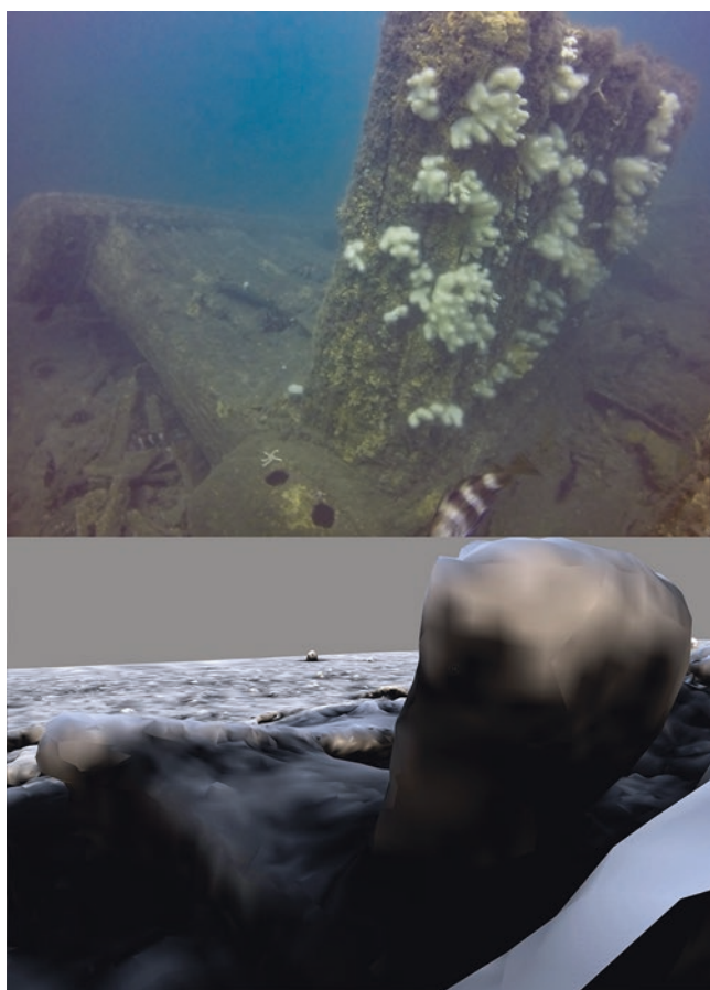
Fig. 12.6 Top: Photograph of one of Falmouth's Y-shaped Yarrow boilers, taken by local diver Mike Radley. (Mike Radley). Bottom: Yarrow Boiler Screenshot. (Maritime and Coastguard Agency © Crown copyright)
