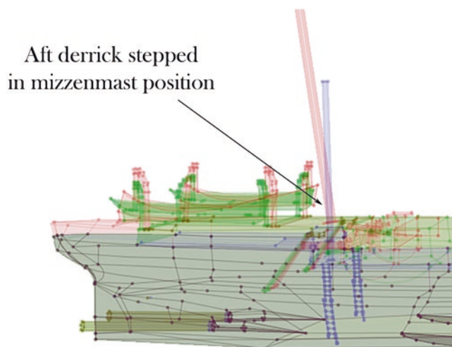
Fig. 6.8 Superimposed digital models of the stern section of Protector / Sidney derived from archival sources, showing the position of the vessel's mizzenmast and aft derrick in its respective colonial navy (red) and civilian (blue) configurations. Grey represents where all models overlap (ACVT/authors)
