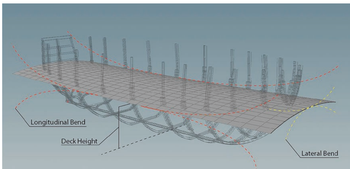
Fig. 8.7 Deck design
