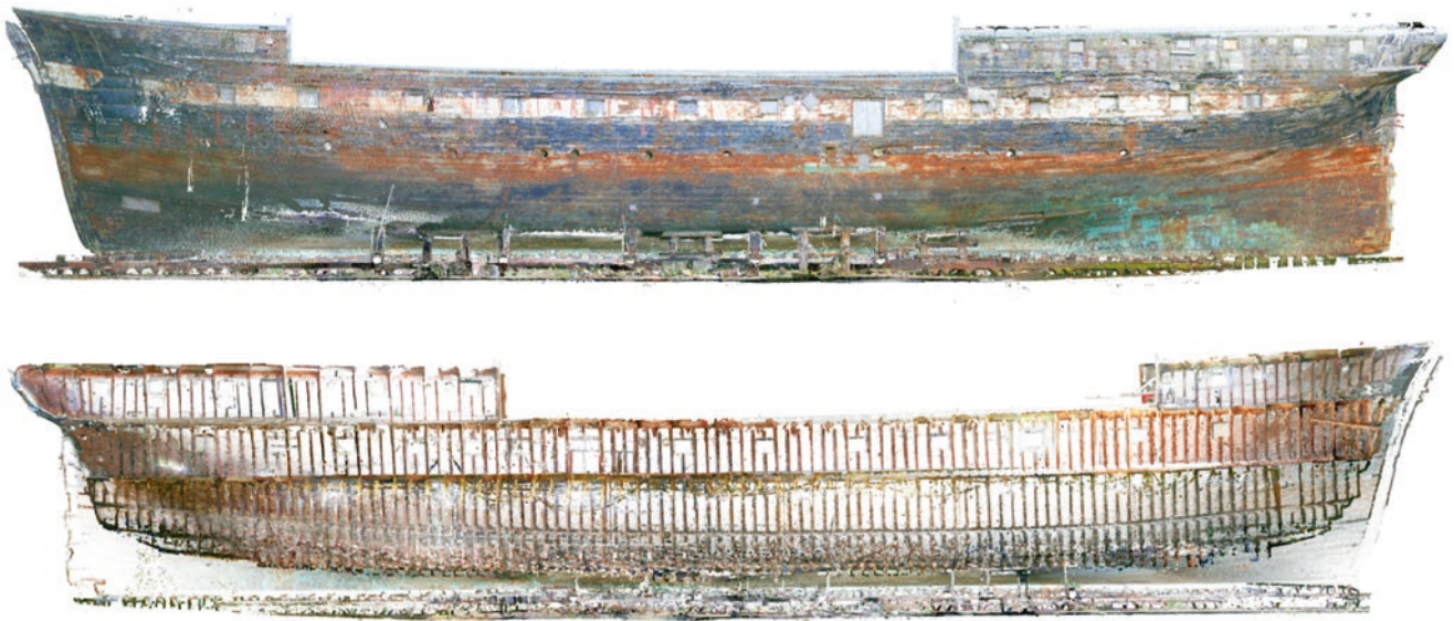
Fig. 7.3 External and internal long sections of the City of Adelaide as acquired from the survey data (Headland Archaeology Ltd)
