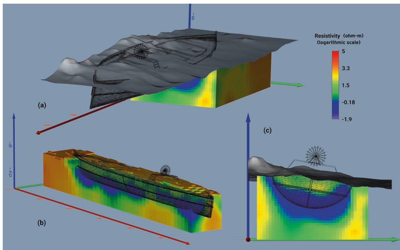
Fig. 11.11 Various views of electrical resistivity data (blue to red colours, representing respectively metallic parts to river sand) with the Crowie model (wireframe representation) submerged under the seabed (gray surface)
