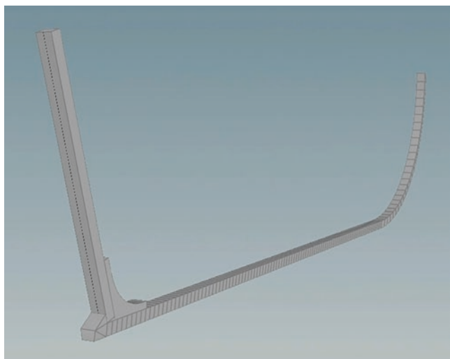
Fig. 8.6 Screen capture showing the model's keel and posts
