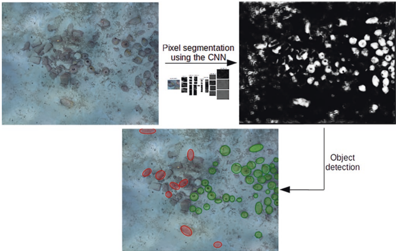
Fig. 9.3 Pixel segmentation on the testing part of the Xlendi orthophoto. On the probability map, the higher the probability of a pixel being an amphora, the higher the probability.
