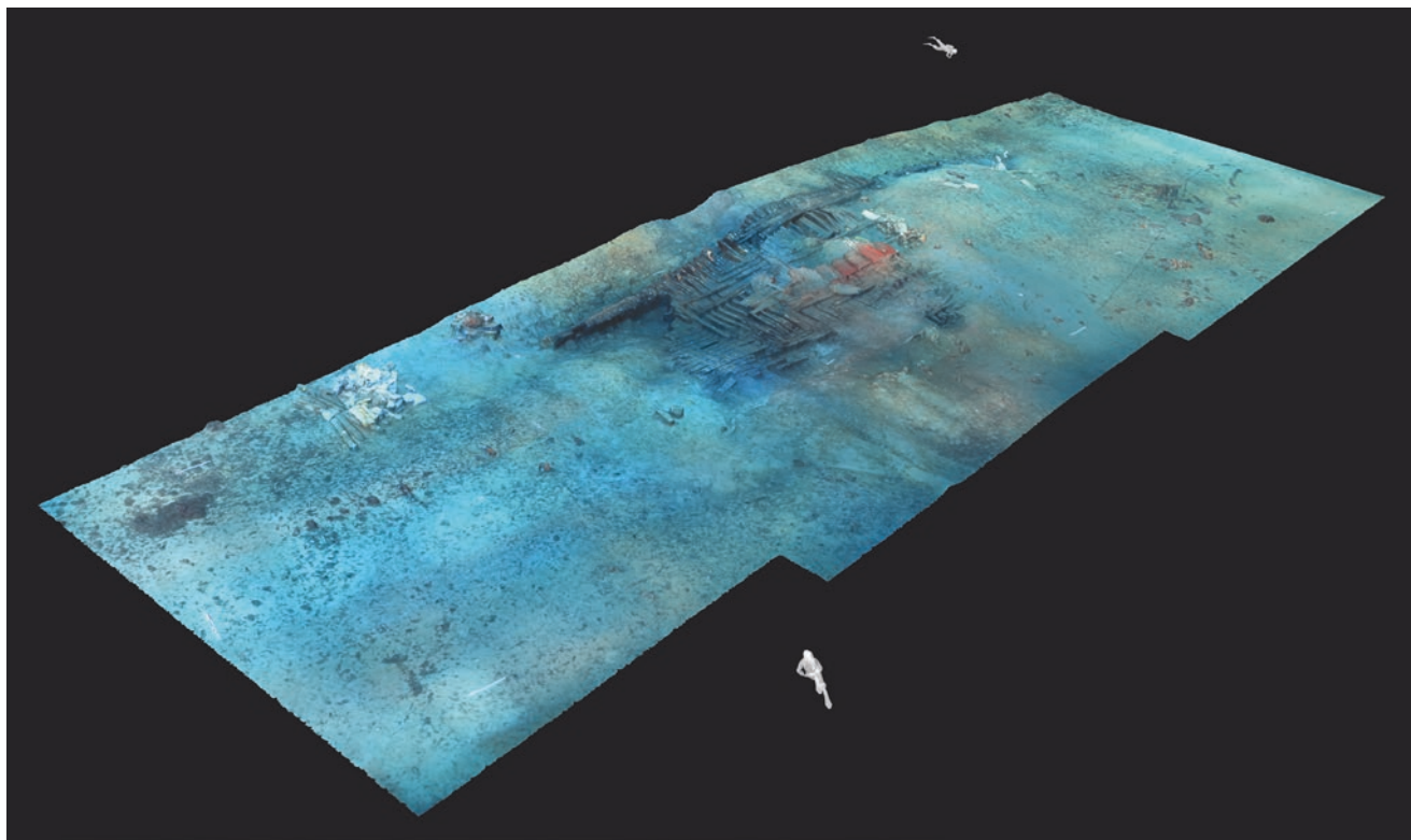
Fig. 4.12 Photogrammetric model of the entire Gnalić shipwreck site. The area measures approximately 60 × 20 m. The model includes further-most stern (rudder pintles?) and bow (grapnel anchor chain?) concretions (K. Yamafune)
