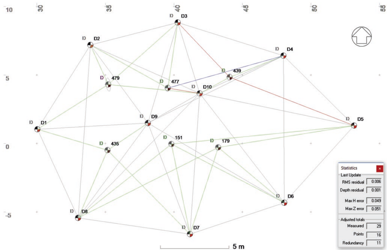
Fig. 4.8 Local coordinate network of the Gnalić shipwreck site (R. Torres, K. Yamafune)
