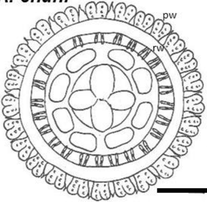
Figure 1.4 Composite drawings of Atolla specimens and photographs depicting key morphological landmarks for species differentiation. Scales marked for each species respectively. See accompanying table (Table 1.1) for further detail. Landmark key: A. wyvillei – te = tentacle, cm = coronal muscle, so = stomach ostia, gs = gastric sinus, go = gonad, rs = radial septa, la = marginal lappet; A. vanhoeffeni – sp = black spots around stomach ostia; A. chuni – pw = pedalial warts, rw = radial warts. Figure continued on following page. Photographs were available only for A. tenella and Super Atolla due to the paucity of data with which to draw composite drawings of the species. This species and potential species nova remain poorly understood and not yet fully documented. Drawings and photographs author's own with the exception of: A. vanhoeffeni photograph (Russell, 1970); A. chuni photograph (Smithsonian, available at: https://www.gbif.org/occurrence/1320668521 );
