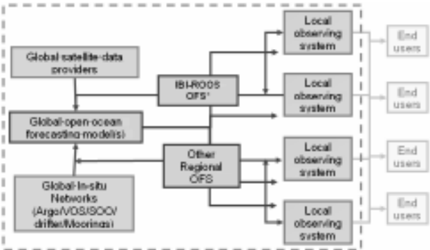
Figure 4 Data sharing with IBI–roos.
