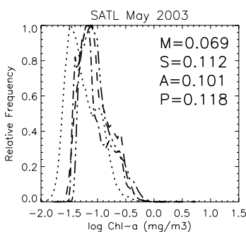
Figure 4 Chl- a South Atlantic Gyrals province distribution functions and corresponding mean values (in \text{mg m}^{-3} ).
