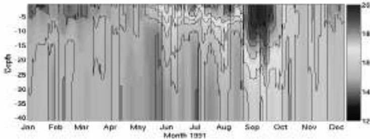
Figure 3 Time evolution of the temperature structure during 1991 simulation, °C.
