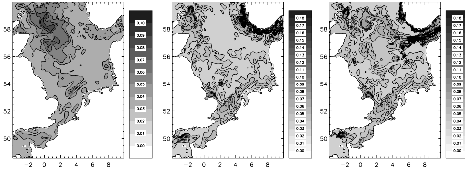
Figure 5 a) Horizontal distribution of rms discrepancy (°C) between temperature modelled without and with data assimilation. Left: at the sea surface for January 2001; Centre: at the sea surface for August 2001; Right: at the sea bed for August 2001.
