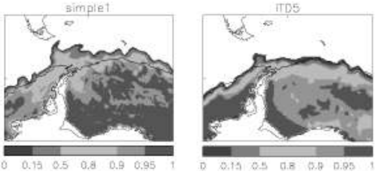
Figure 5 FOAM sea–ice concentration fields in the Drake passage for simple ice advection (left panel) and for the EVP and ITD ice model (right panel). The black line is an ice edge analysis.
