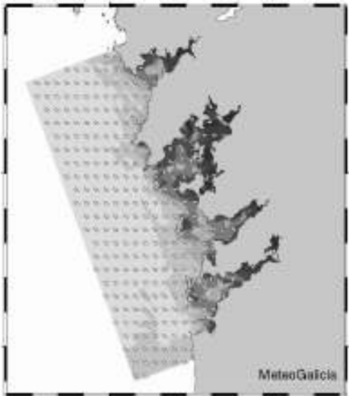
Figure 2 Plot of significant wave height (background tint) and mean wave direction (arrows) for Rias Baixas model grid.
