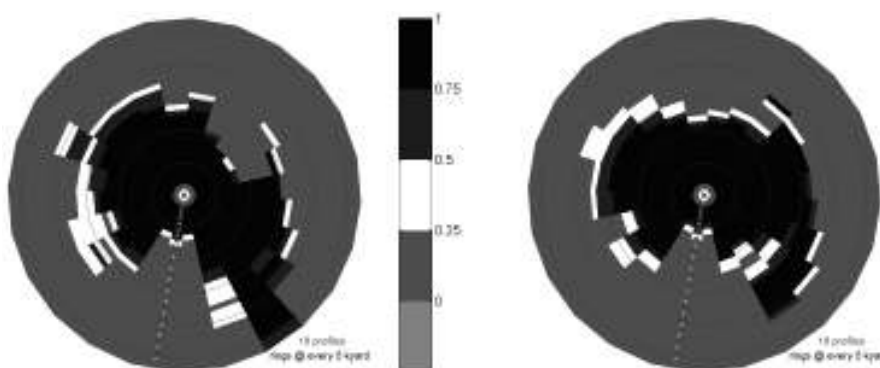
Figure 6 Sonar performance for position C, based on forecasts of 10 April 2004 after 00 and 84 hours. The overall performance at this position is worse, because a muddy seafloor is assumed here (coarse sand at position A).
