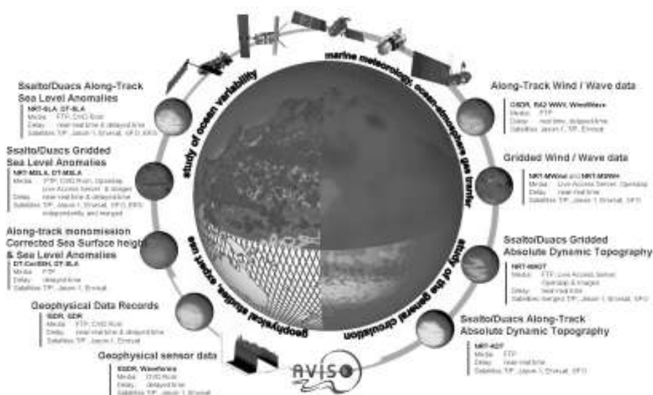
Figure 1 A whole constellation of data products from ocean altimetry satellites, including multi-mission products, available along-track and gridded, in delayed and near-real time, for different uses (oceanography, geophysics, meteorology, operational, etc.), for different users (from experts to newcomers), and on different media (DVD, FTP, web interactive interfaces, etc.)
