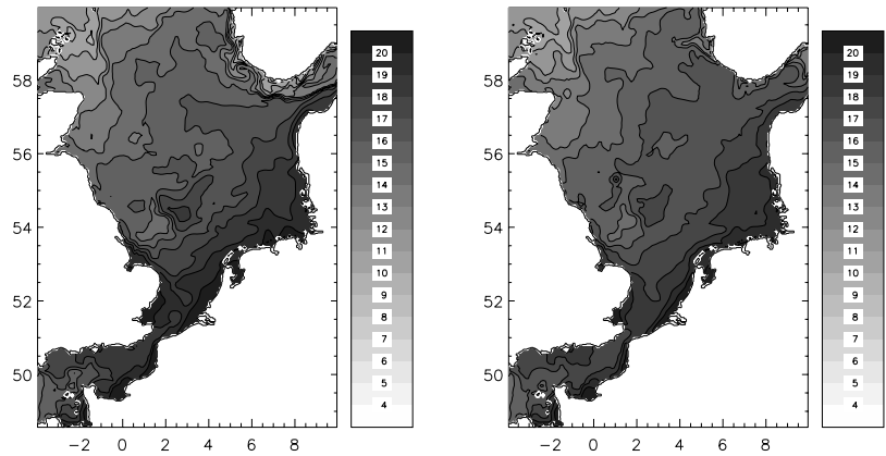
Figure 1 Horizontal distribution of modelled temperature (°C) at the sea surface on 15 August 2001. Left: without data assimilation; Right: with data assimilation.
