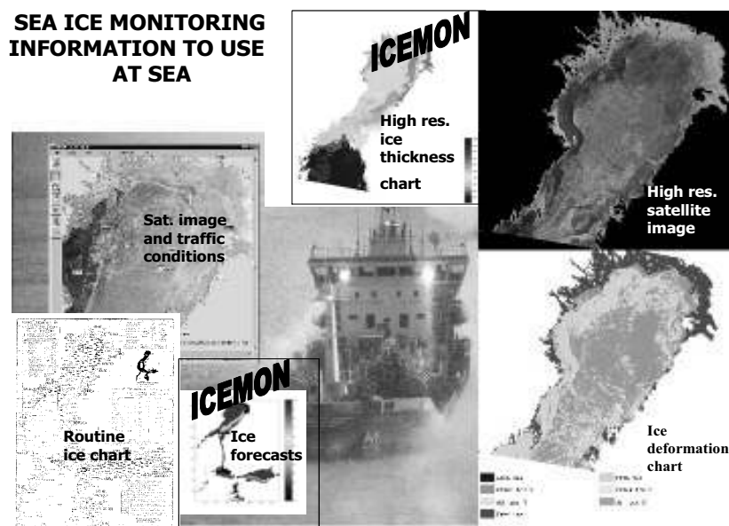
Figure 1 Set of ice information available to users at sea from the Finnish Ice Service. High-resolution ice thickness charts and ice forecasts were ICEMON products and services.
