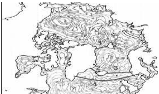
Figure 1 Chosen sections for research and comparison 1–Fram Strait; 2–Dutch Strait; 3–Section between Norway and Iceland; 4–60°N.
