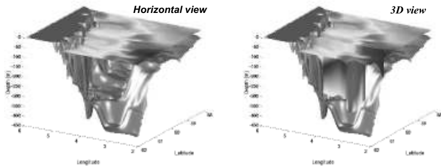
Figure 2 Selected view of the temperature field (light grey indicate cold water) provided by the MONCOZE system as seen from northwest (depicting the Norwegian Trench along the west coast of Norway). Left: horizontal temperature structure at 50 m. Right: vertical temperature structure across the Norwegian Trench displayed together with the horizontal temperature.
