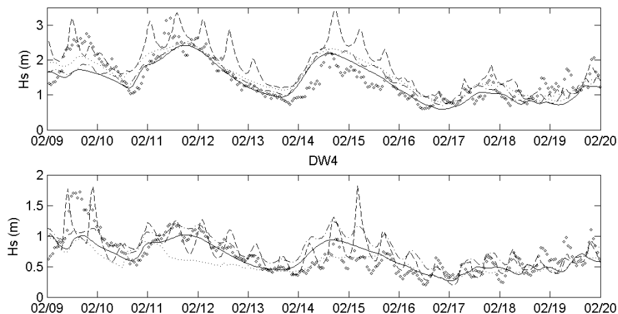
Figure 3 Tidal influence on wave propagation. Diamonds: measurements, continuous/dotted lines: TOMAWAC/SWAN without tidal effect, Dot-dashed/dashed lines: TOMAWAC/SWAN with tidal effects.
