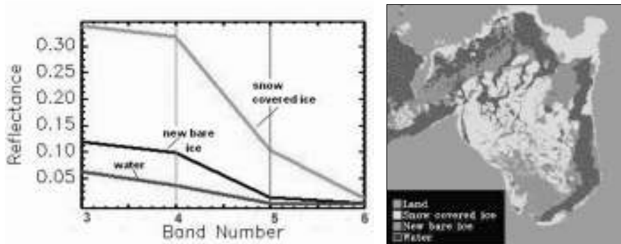
Figure 2 Left: Spectral shape of snow covered ice, new bare ice and water. Right: Ice types in Gulf of Riga on 11 March 2003.
