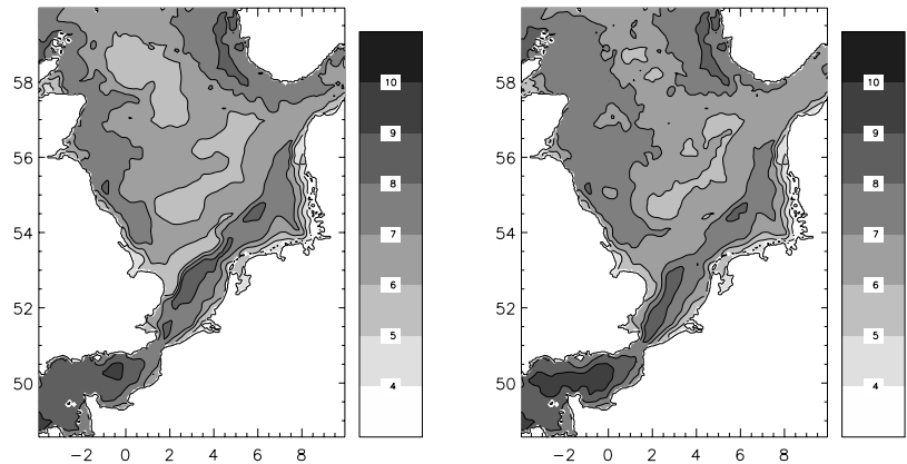
Figure 2 Horizontal distribution of modelled temperature (°C) at the sea surface on 15 January 2001. Left: without data assimilation; Right: with data assimilation.
