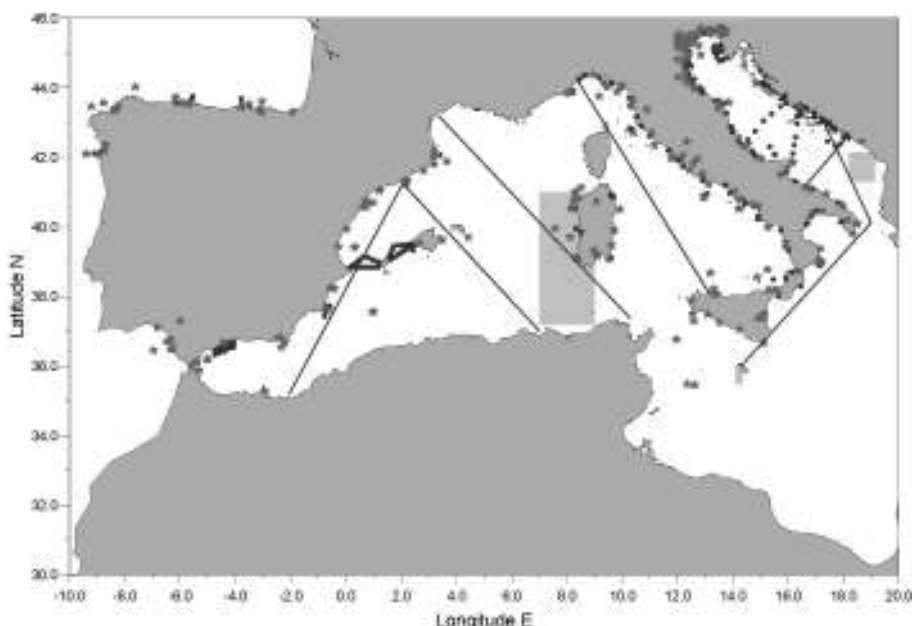
Figure 1 Spatial coverage of ocean-observing systems in the Central and Western Mediterranean.
