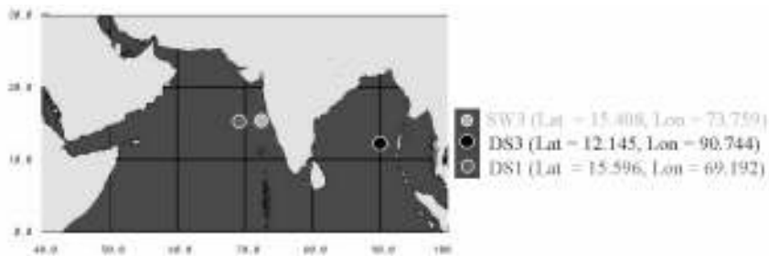
Figure 2 Location of Indian buoys.
