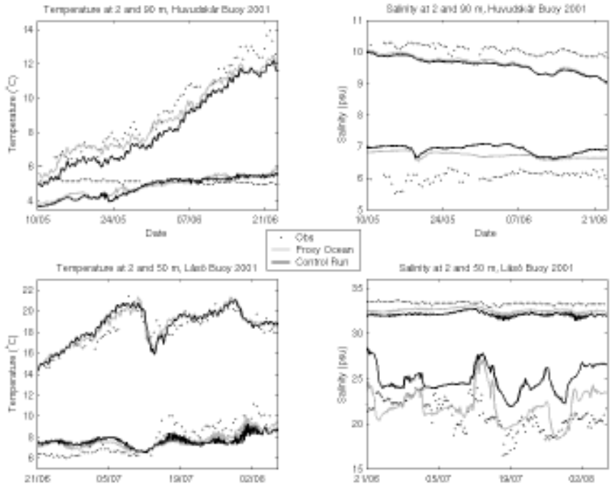
Figure 4 Surface and bottom temperature (left) and salinity (right) in the Baltic Sea at 19 11 E 58 56 N (upper panel) and in Kattegat at 11 32 E 57 12 N (lower panel). See caption legend for details.
