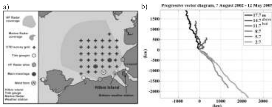
Figure 1 a) Location map showing measurements, b) progressive vector diagram, 7 August 2002 to 12 May 2005.
