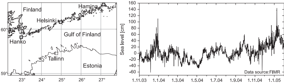
Figure 1 Sea level observation sites at the Finnish coast of the Gulf of Finland and the sea level in Helsinki from November 2003 to January 2005. Reference level: Finnish geodetical height system N60.
