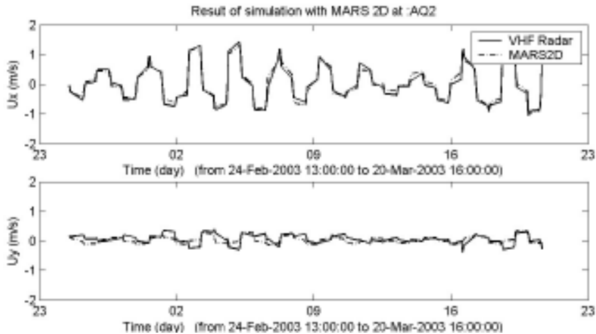
Figure 2 Comparison between simulations with MARS-2D and measurement at AQ2 position.
