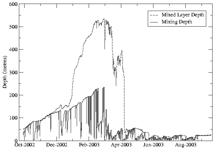
Figure 4 Time evolution of Kraus-Turner mixing depth (solid line) and diagnostic mixed layer depth (dotted line).
