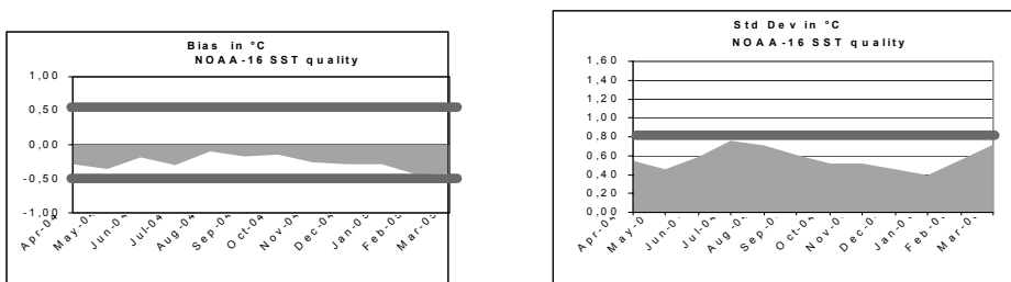
Figure 8 NOAA-16 NAR SST Quality results over the period April 2004–March 2005. The results show the bad impact of a recurrent technical problem onboard the satellite.
