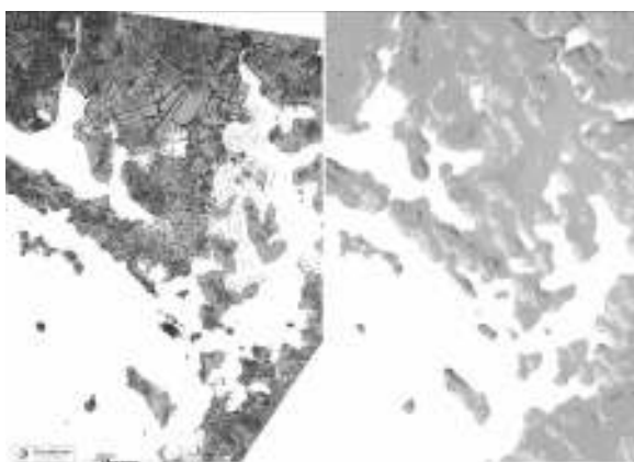
Figure 2 Left: a lidar topographic model (showing relief and some coverage of vegetation and buildings, cell size = 2 m, \sigma_Z : 15 cm). Right: an IGN BDAI™ DTM derived from photogrammetric restitution (relief, without any vegetation or buildings informations, cell size = 50 m, \sigma_Z = 2 m). Shading is used to highlight the texture of the relief and exaggerates the differences between flat and step areas.
