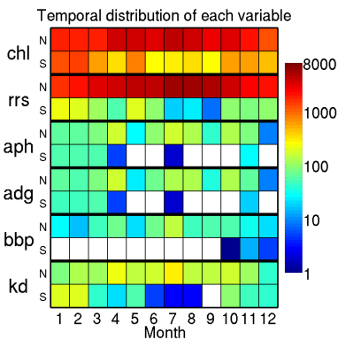
Figure 3. Temporal distribution of chlorophyll a concentration (chl), remote-sensing reflectance (rrs), algal pigment absorption coefficient (aph), detrital plus CDOM absorption coefficient (adg), particle backscattering coefficient (bbp) and the diffuse attenuation coefficient for downward irradiance (kd) in the final table. All chlorophyll data were considered, but for a given station HPLC data were selected if available. Colours indicate the number of stations available for each variable, as a function of months and the hemispheres of data acquisition (N – Northern Hemisphere; S – Southern Hemisphere).
