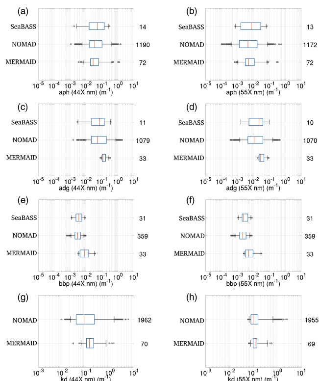
Figure 12. The distribution of (a) aph at 44X nm, (b) aph at 55X nm, (c) adg at 44X nm, (d) adg at 55X nm, (e) bbp at 44X nm, (f) bbp at 55X nm, (g) kd at 44X nm and (h) kd at 55X nm. Data were first searched at 445 and 555 nm and then with a search window of up to 8 nm to include data at 547 nm. The graphical convention is identical to Fig. 2.
