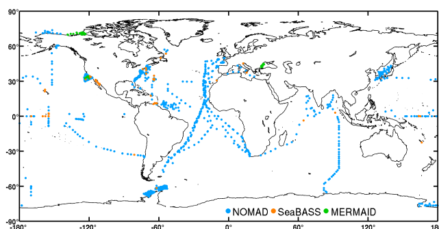
Figure 15. Global distribution of diffuse attenuation coefficient for downward irradiance ( \text{kd} ) per dataset in the final table.
