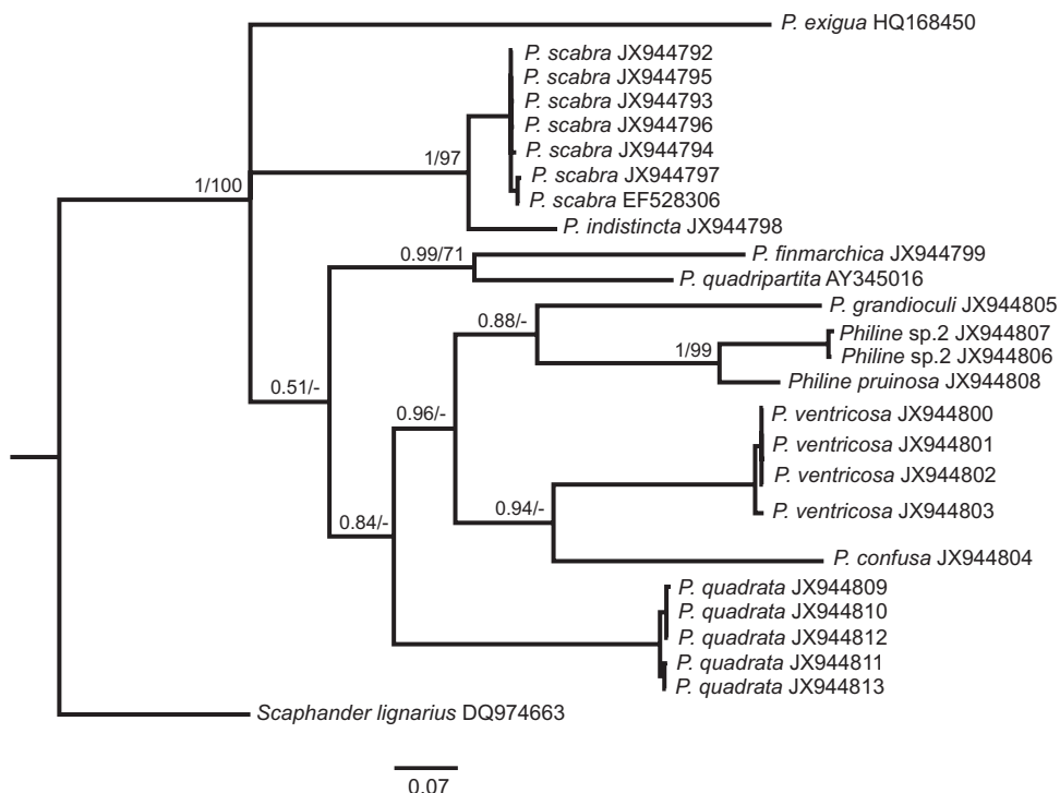
Figure 33. Phylogenetic hypothesis for Philine species based on Bayesian inference analysis of mitochondrial cytochrome c subunit I gene sequences. Numbers above branches represent posterior probabilities (on left side of dashed line) and parsimony bootstrap support (on right side of dashed line).
