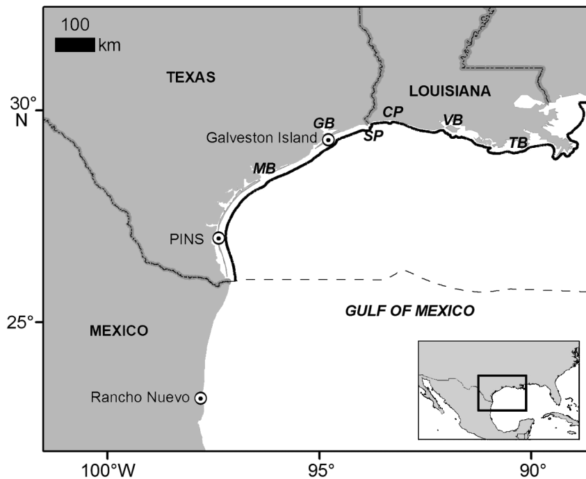
Fig. 1. Western Gulf of Mexico showing the location of Rancho Nuevo, Tamaulipas, Mexico; Padre Island National Seashore (PINS), North Padre Island, Texas; and Galveston Island, Texas, USA, as well as selected bays and passes: Matagorda Bay (MB), Galveston Bay (GB), Sabine Pass (SP), Calcasieu Pass (CP), Vermilion Bay (VB), and Timbalier Bay (TB). The solid black line marks the offshore extent of Texas and Louisiana state waters; the dashed black line marks the offshore extent of US territorial waters (Exclusive Economic Zone)
