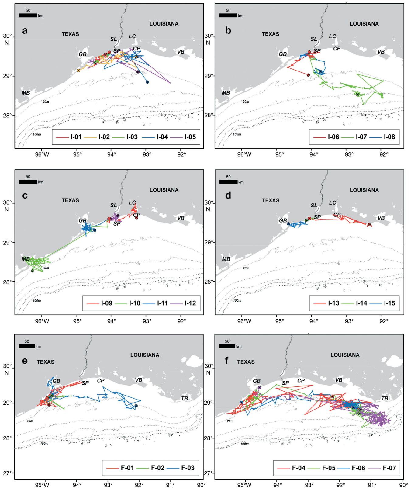
Fig. 2. Lepidochelys kempii . Filtered satellite tracks. ⊙: Release and ⊗: end of track. Immature individuals tracked during (a) 2004 to 2005, (b) 2006, and (c,d) 2007, and adult females tracked during (e) 2005 and (f) 2006 to 2007. MB: Matagorda Bay; GB: Galveston Bay; SL: Sabine Lake; SP: Sabine Pass; LC: Lake Calcasieu; CP: Calcasieu Pass; VB: Vermilion Bay; TB: Timbalier Bay. The gray dashed lines depict the 20 m through 100 m isobaths, in 20 m increments
