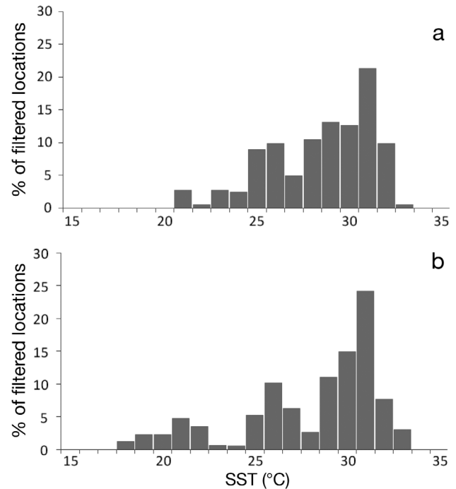
Fig. 4. Lepidochelys kempii . Advanced Very High Resolution Radiometer (AVHRR) sea surface temperature (SST) distributions for (a) 15 immature ridleys (404 locations) and (b) 7 adult female ridleys (769 locations). Sea surface temperature (SST) data were not available for all accepted locations
