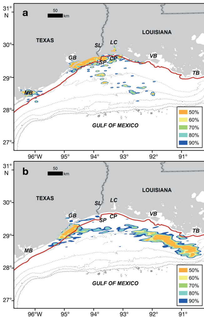
Fig. 5. Lepidochelys kempii . Use of the northwestern Gulf of Mexico, as estimated with kernel density estimation (KDE) by (a) 15 immature ridleys (358 average daily locations) and (b) 7 adult female ridleys (508 average daily locations). MB: Matagorda Bay; GB: Galveston Bay; SL: Sabine Lake; SP: Sabine Pass; LC: Lake Calcasieu; CP: Calcasieu Pass; VB: Vermilion Bay; TB: Timbalier Bay. The solid red lines mark the offshore extent of Texas and Louisiana state waters. The gray dashed lines depict the 20 m through 100 m isobaths, in 20 m increments
