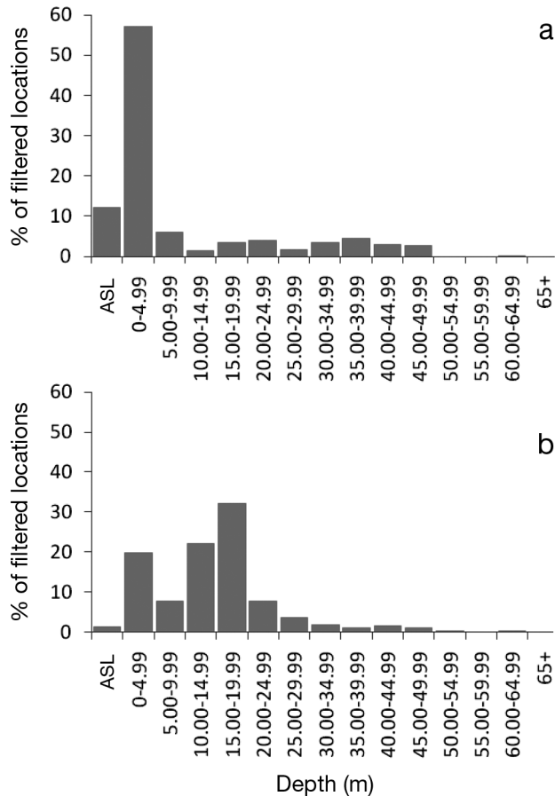
Fig. 3. Lepidochelys kempii . Water depth distributions of (a) 15 immature ridleys (591 locations) and (b) 7 adult female ridleys (887 locations). Depth values above sea level (ASL) represent primarily coastal lakes or bays
