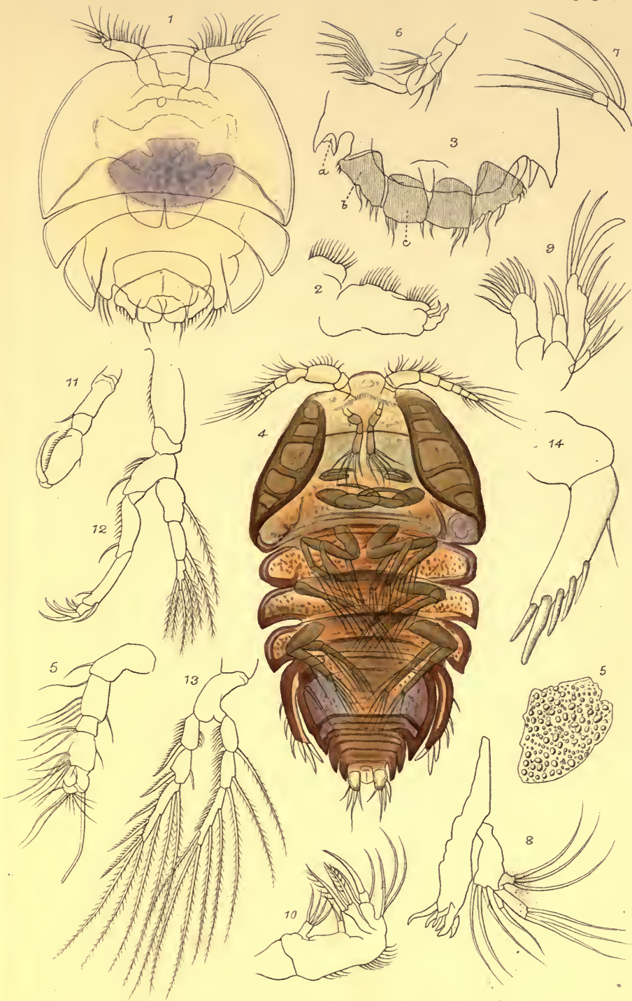
1-3 Porcellidium subtrotundum . 4-15 Peltidium interruptum .
