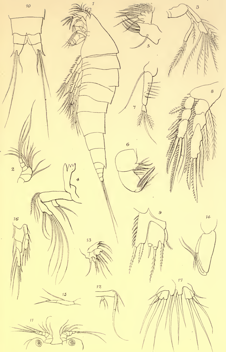
1-10 Ectinosoma spinipes . 11-17 " " erythropus .
