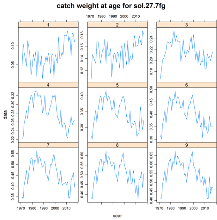
Figure 1. Catch weight-at-age.
