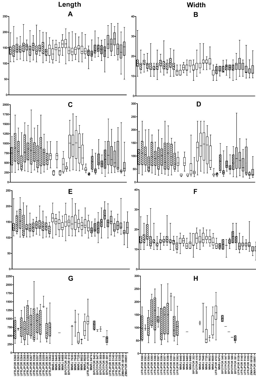
Figure 7. Box-and-whisker plot (maximum and minimum size; upper and lower quartiles and median) of spicule size of Leucetta spp. A, triactine I length; B, triactine I width; C, triactine II length; D, triactine II width; E, tetractine I length; F, tetractine I width; G, tetractine II length; H, tetractine II width. ▨ Leucetta floridana (Caribbean), □ Leucetta floridana (Brazil), ▩ Leucetta sp., ▤ Leucetta microraphis .
