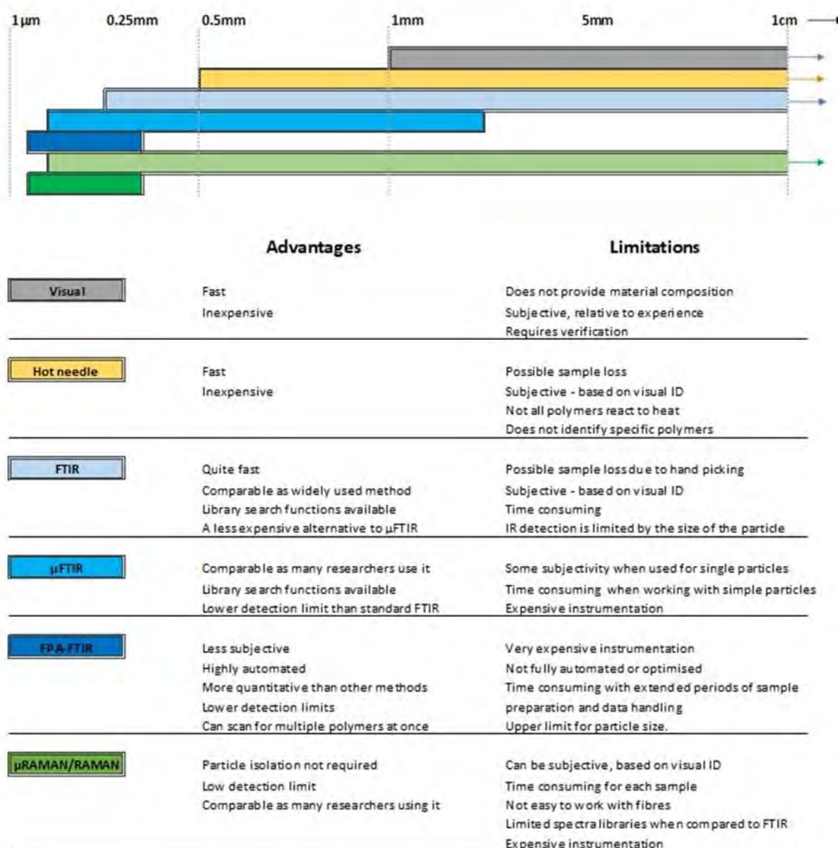
Figure 3.1.3-1 Methods used for the identification and subsequent verification of plastic particles from different size ranges.
