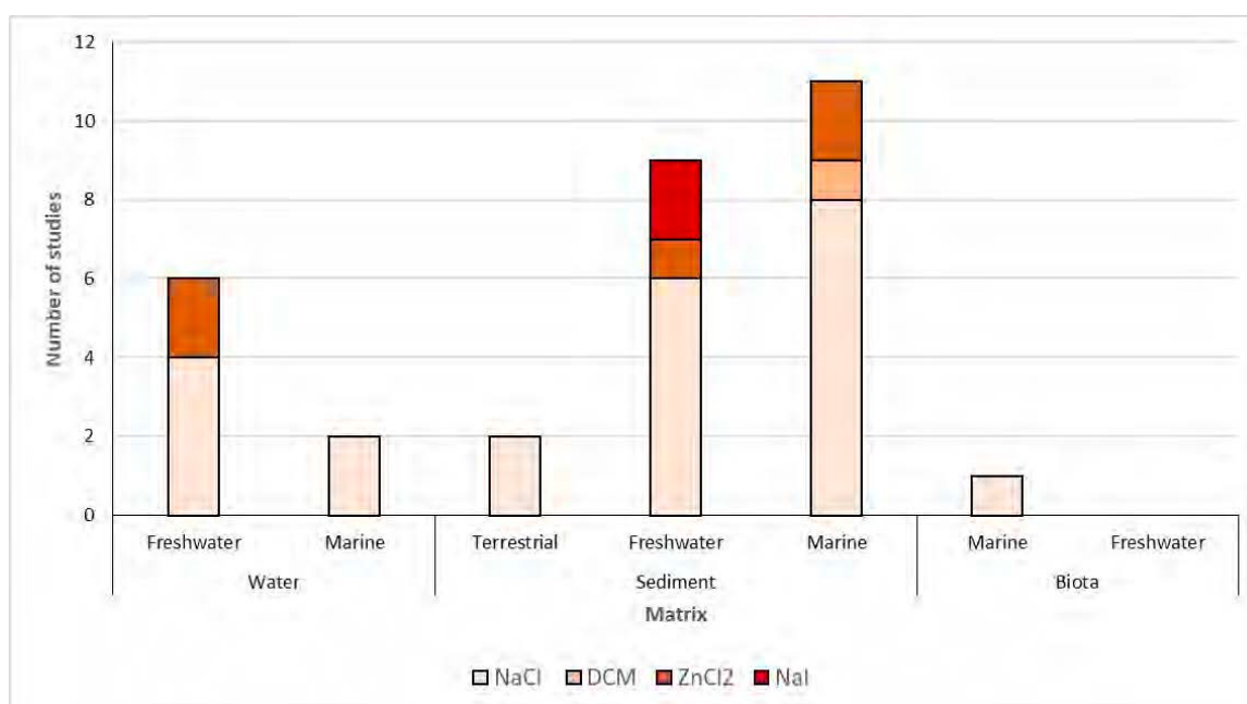
Figure 3.1.2-2 The use of different density solutions for processing environmental matrices. NaI = sodium iodide, DCM = dichloromethane, ZnCl 2 = zinc chloride, NaCl = sodium chloride
