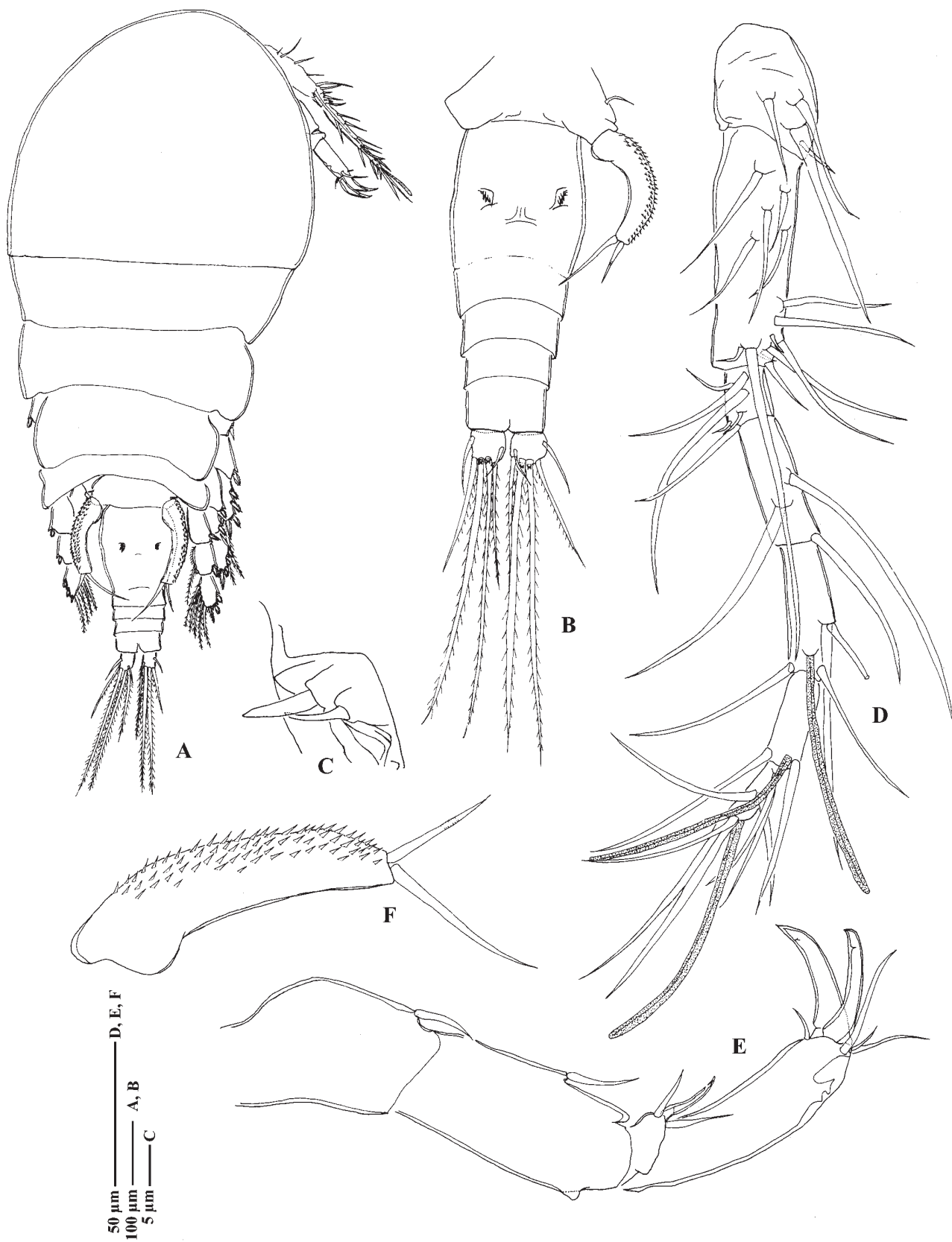
FIG. 3. – Doridicola comai , sp. nov. Female. A, habitus, dorsal; B, urosome, dorsal; C, genital area; D, antennule; E, antenna; F, free segment of leg 5.
