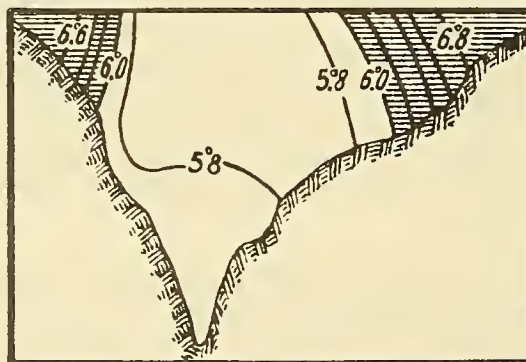
Figure 13. The arrangement of isotherms in the Gorlo Belogo Morya in August.
