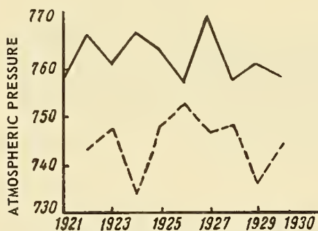
Figure 28. Mean atmospheric pressure in December at Cape Barrow (—) and mean atmospheric pressure in December at the center of the Iceland minimum (--).
