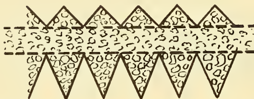
Figure 102. An isostatically balanced hummock field.
