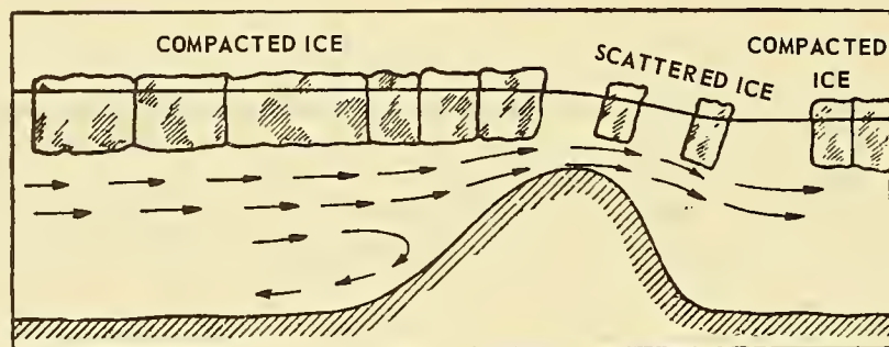
Figure 125. Thinning of ice behind shoals.
