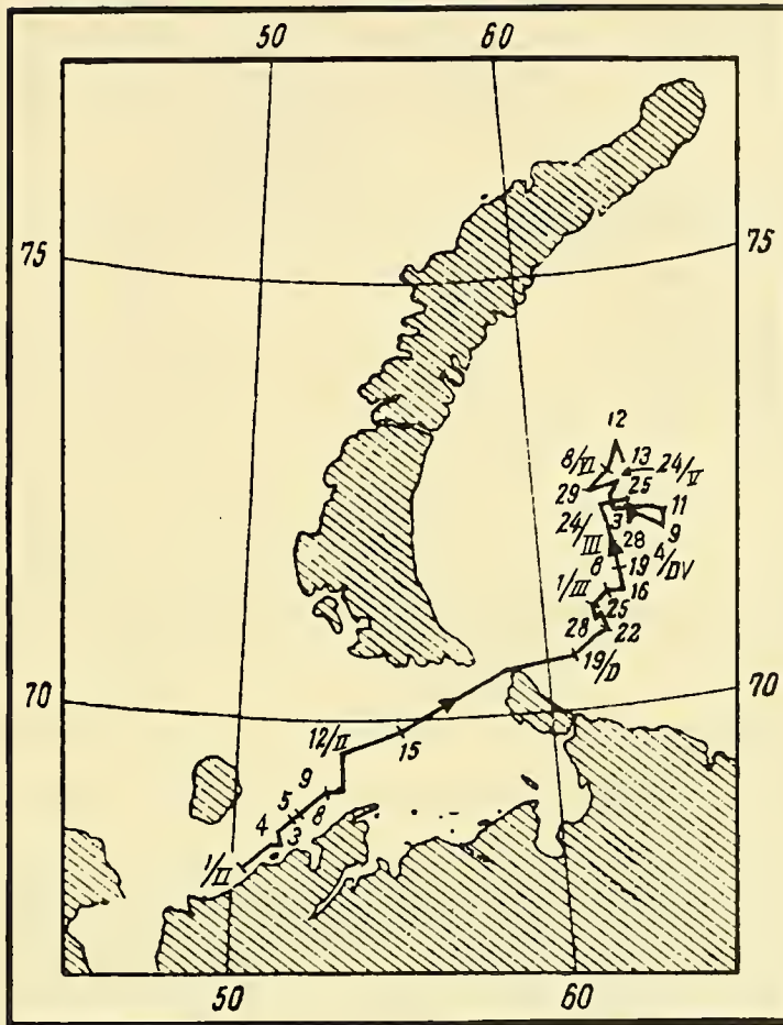
Figure 159. Drift of the Solouei-Budimirovich .
