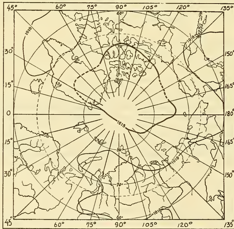
Figure 164. Average atmospheric pressure for April through June, 1938 to 1939.
