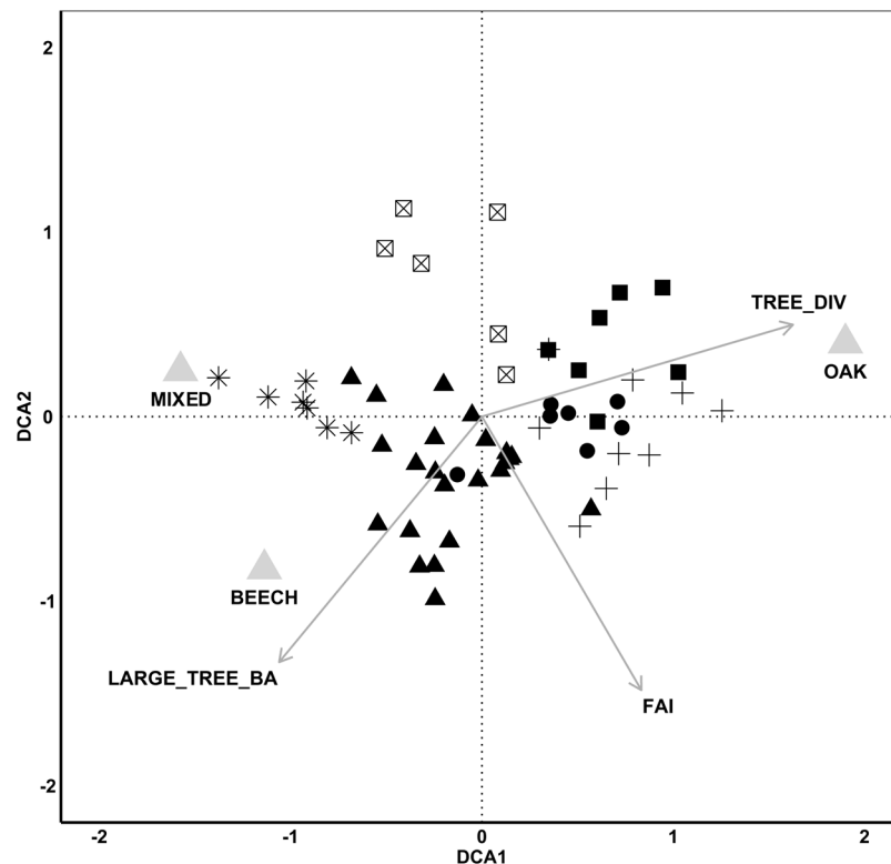
Figure 3 – DCA of the 59 plots. Only first 2 axes are presented and only significant environmental factors according to CCA are passive projected onto DCA ordination. Fungal assemblages are symbolized according to their classification in hierarchical clustering: black triangle = Cluster 1; star = Cluster 2; crossed-square = Cluster 3; black square = Cluster 4; black circle = Cluster 5; cross = Cluster 6. Eigenvalues: Axis 1 – 0.2617, Axis 2 – 0.1629. Length of gradient along Axis 1 – 2.63.
