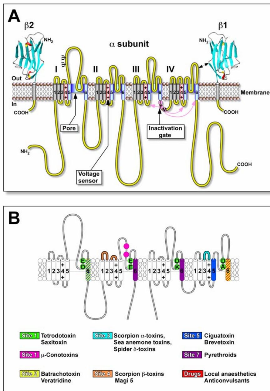
Figure 2. Molecular structure and neurotoxin receptor sites of the Na v channel. (A) Schematic representation of the subunit structure of the Na v channel showing the functional \alpha -subunit and ancillary \beta -subunits. Cylinders represent the \alpha -helical segments where the charged S4 segments (red) represent the voltage sensors. The inactivation gate (magenta) is represented by the inactivation particle (residues IFM). The walls of the ion-conducting pathway are shown in blue. The \beta 1 and \beta 2 subunits are represented as immunoglobulin-like folds similar to myelin protein P 0 [111]. \Psi , sites of probable N-linked glycosylation. (B) Location of known neurotoxin receptor sites on Na v channels. Green circles represent the outer (EEDD) and inner (DEKA) rings of amino acid residues that form the ion selectivity filter and the proposed neurotoxin receptor site 1 for the water-soluble guanidinium.
