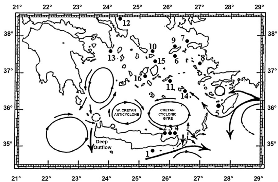
Fig. 1: Sampling stations in the Aegean Sea (basic map from SOUVERMEZOGLOU et al. , 1999).
