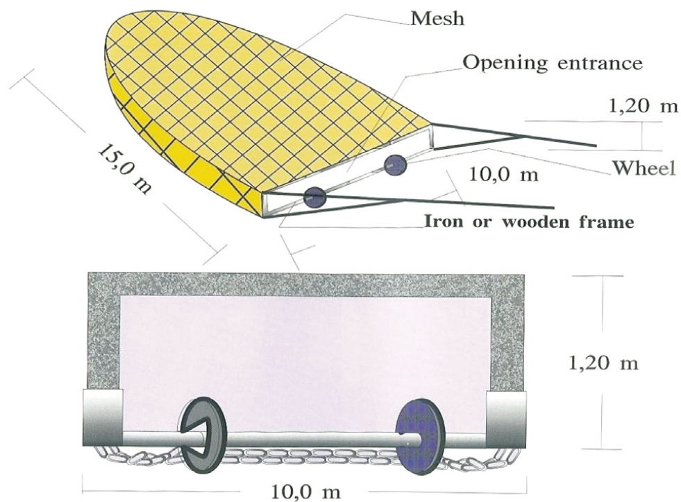
Fig. 2: Schematic depiction of gagava.
