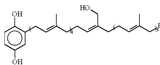
Hydroquinone B 2-(24hydroxy) Octaprenylo 1,4 hydroquinone
