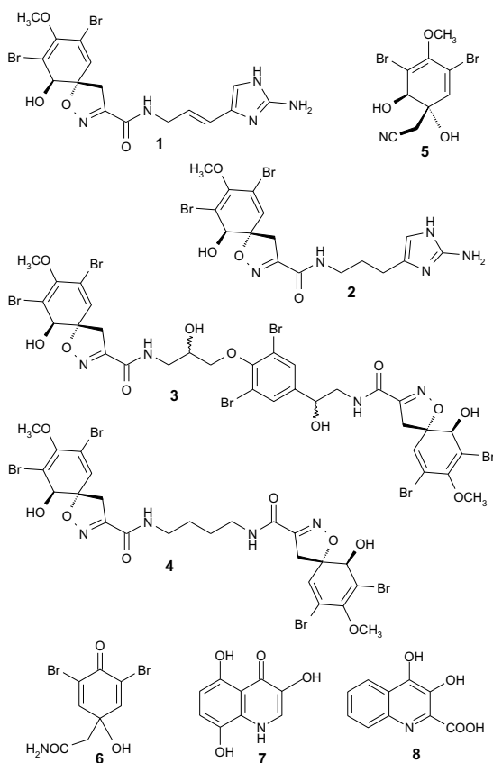
Fig. 3. Structures of Aplysina alkaloids: aplysinamisins-1 ( 1 ), aerophobin-2 ( 2 ), isofistularin-3 ( 3 ), aerothionin ( 4 ), aeroplysinin-1 ( 5 ), dienone ( 6 ), uranidine ( 7 ), and 3,4-dihydroxyquinoline-2-carboxylic acid ( 8 ).
