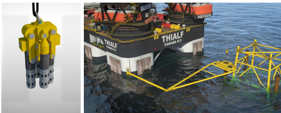
Fig. 16. Concept of push-in piles with specific tool (left). Helical piles as jacket pinpile with rotating tool (right), © Heerema Marine Contractors.
