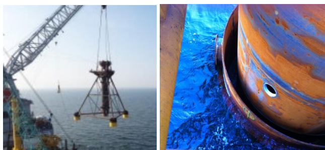
Fig. 6. Cofferdam application with monopile (left: Aarhus Bight, right: OWF Anholt) ©K.E. Thomsen
