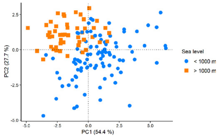
Fig. 6. PCA of morphometric measurements and parameters of 142 individuals of Clausilia dubia highlighting geographic regions (above) and sea level (below). GUT = Gutenstein Alps, RSG = Rax-Schneeberg Group, RGM = Prealps east of the Mur, WAU = Wachau, WAV = Waldviertel, WIW = Wienerwald, YBB = Ybbstal Alps.
