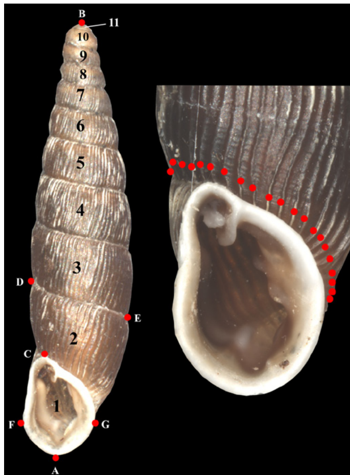
Fig. 2. Landmarks for morphometric measurements (red dots; for better visibility enlarged). Left: numbering of whorls ( C. d. gracillior ). A–B: shell height, A–C: aperture height, D–E: shell width, F–G: aperture width. right: marking of ribs along the aperture ( C. d. dubia ).
