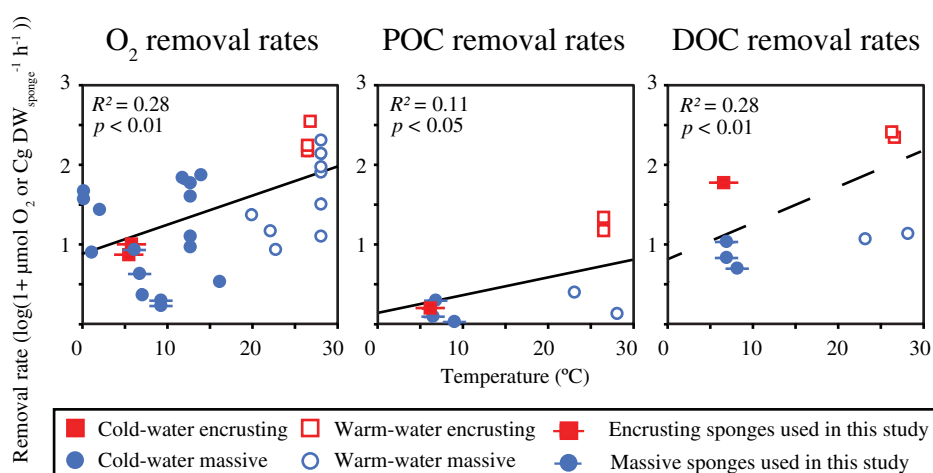
Fig. 4. Oxygen, particulate, and dissolved organic carbon (POC and DOC) removal rates for cold-water ( < 15^{\circ}C ) and warm-water ( > 15^{\circ}C ) marine sponges plotted against temperature. Removal rates are log transformed. Red squares depict encrusting sponges, blue circles depict massive sponges (i.e., all non-encrusting growth forms). R^2 values are based on the linear regression of all values (encrusting + massive). Regression lines are given by \log(1 + \mu\text{mol } O_2 \text{ g DW}_{\text{sponge}}^{-1} \text{ h}^{-1}) = 0.033 * T(^{\circ}C) + 0.90 , \log(1 + \mu\text{mol POC g DW}_{\text{sponge}}^{-1} \text{ h}^{-1}) = 0.017 * T(^{\circ}C) + 0.21 and \log(1 + \mu\text{mol DOC g DW}_{\text{sponge}}^{-1} \text{ h}^{-1}) = 0.041 * T(^{\circ}C) + 0.77 . All non-log-transformed rates are given in Table S2.
