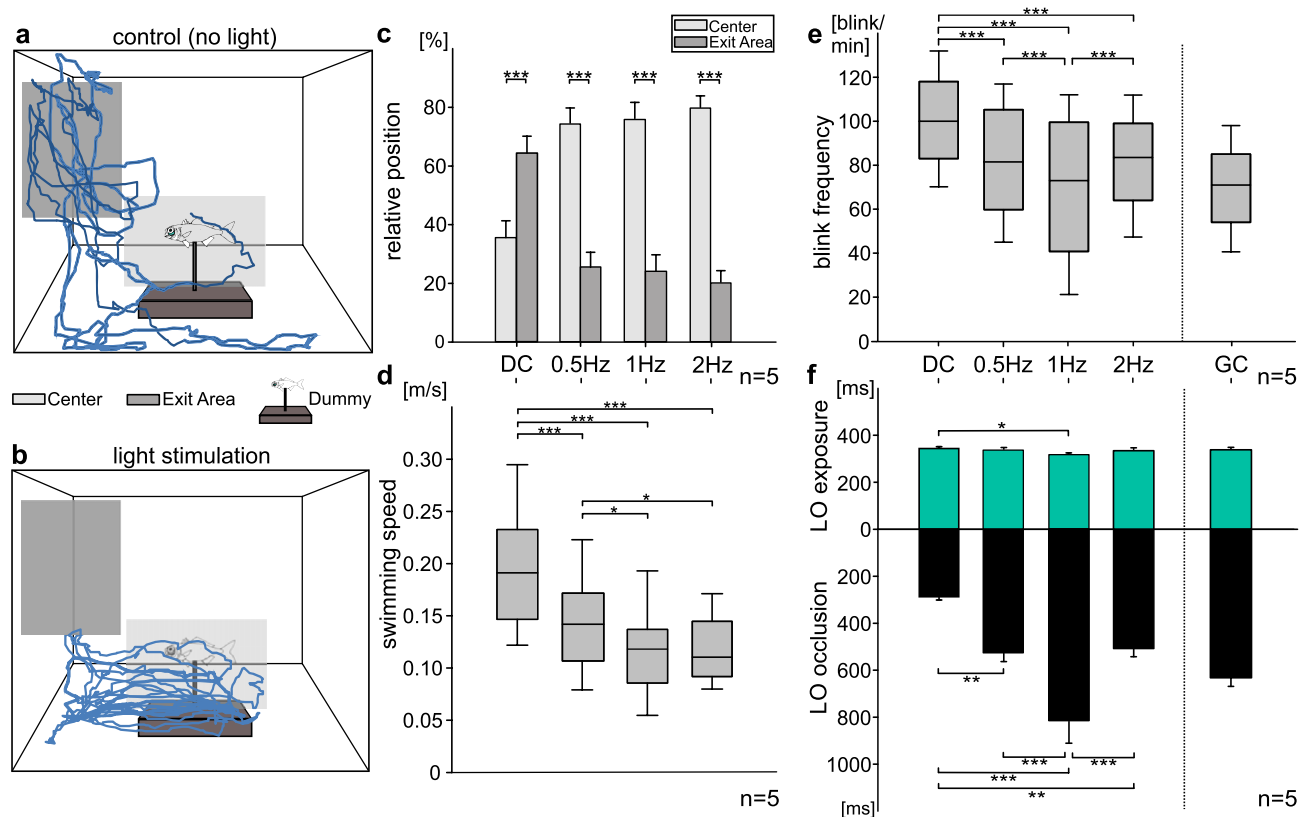
Figure 1. Frequency-dependent light stimuli transmitted by artificial light organs mediate changes in positioning, swimming speed, blink frequency and light organ occlusion of A. katoptron . (a,b) Example trajectories of A. katoptron (60 s) without (a) and with (b) a 1 Hz light stimulation of the fish dummy. (c) Relative positioning in exit or center area of isolated A. katoptron during different light stimuli (DC; 0.5, 1, 2 Hz) (n=5). (d) Swimming speed of isolated A. katoptron during different light stimuli (DC; 0.5, 1, 2 Hz) (n=5). (e) Blink frequencies of isolated A. katoptron induced by different light stimuli (DC; 0.5, 1, 2 Hz) (left) in comparison to blink frequencies detected in a small group of five individuals in the reef tank (GC) (right) (n=5). (f) Mean light organ exposure and occlusion times during different light stimuli (DC, 0.5, 1, 2 Hz) (left) in comparison to exposure and occlusion times measured in a small group of five individuals in the reef tank (GC) (right) (n=5). Figures were created with SigmaPlot 12.0 ( www.sigmaplot.co.uk ) and processed with CorelDraw Graphics Suite 2017 ( www.coreldraw.com ). DC, dark control; GC, group control. Significance values are reported as * p < 0.05 , ** p < 0.01 , *** p < 0.001 . Error bars indicate \pm SEM.
