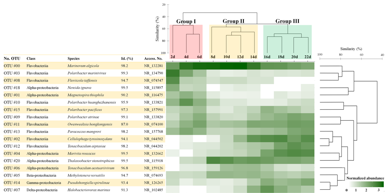
Figure 2. Heatmap showing the most abundant bacterial operational taxonomic units (OTUs). Each OTU displayed a relative abundance of > 1% in at least one sample. The heatmap displayed the fourth root-normalized data at the range of 0.0 to 3.0. Hierarchical agglomerative clustering using the group average of the most abundant bacterial OTUs using the Bray–Curtis similarity method. This figure was generated with RStudio v.1.2.5042 ( https://rstudio.com ).
