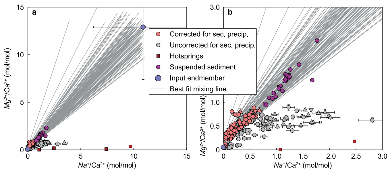
Extended Data Fig. 6 | Mixing diagram for weathering contributions. a , Mg^{2+}/Ca^{2+} – Na^{+}/Ca^{2+} mixing diagram showing raw data (grey) and weathering contributions (red). Blue points mark endmembers with two standard deviations. Dark-red squares are available hot spring data. Purple points are the suspended sediment data from the Chenyulan. The grey lines are the best fit endmember mixing lines found by the inverse approach. b , Close-up of panel a. Symbols mark dominant lithology (see Fig. 1). Error bars are equivalent to a 95% confidence interval.
