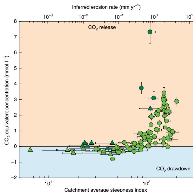
Fig. 4 | Impact of erosion on the long-term carbon cycle. Moles of \text{CO}_2 emitted or sequestered per volume of water against catchment-averaged steepness index (lower x axis) and inferred erosion rates (upper x axis). Symbols mark dominant lithology (see Fig. 1). Error bars are equivalent to a 95% confidence interval. Samples with anomalously high sulfate concentrations are marked as darker points.
