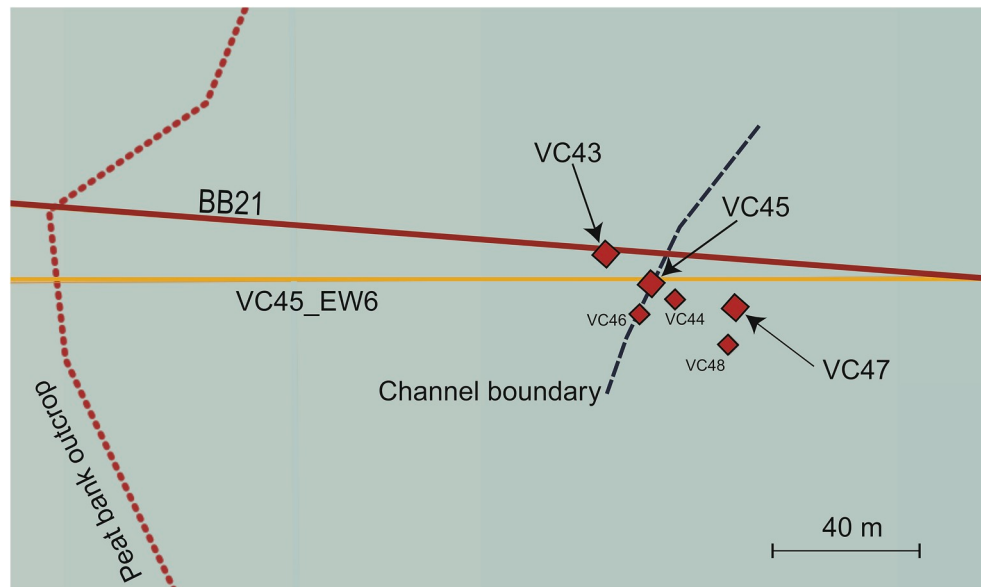
Fig. 5. Top: overview of seismic lines and cores at site VC 43. The red dashed line marks peat outcrop at the seabed. The black dashed line marks the channel boundary. Bottom: Seismic line VC45_EW6 demonstrates that the key peat bed could be linked to material recovered in vibrocore VC45, where a C14 date of 9972 \pm 23 BP (SUERC 89491) has been obtained for the peat bed. (For interpretation of the references to colour in this figure legend, the reader is referred to the Web version of this article.)
