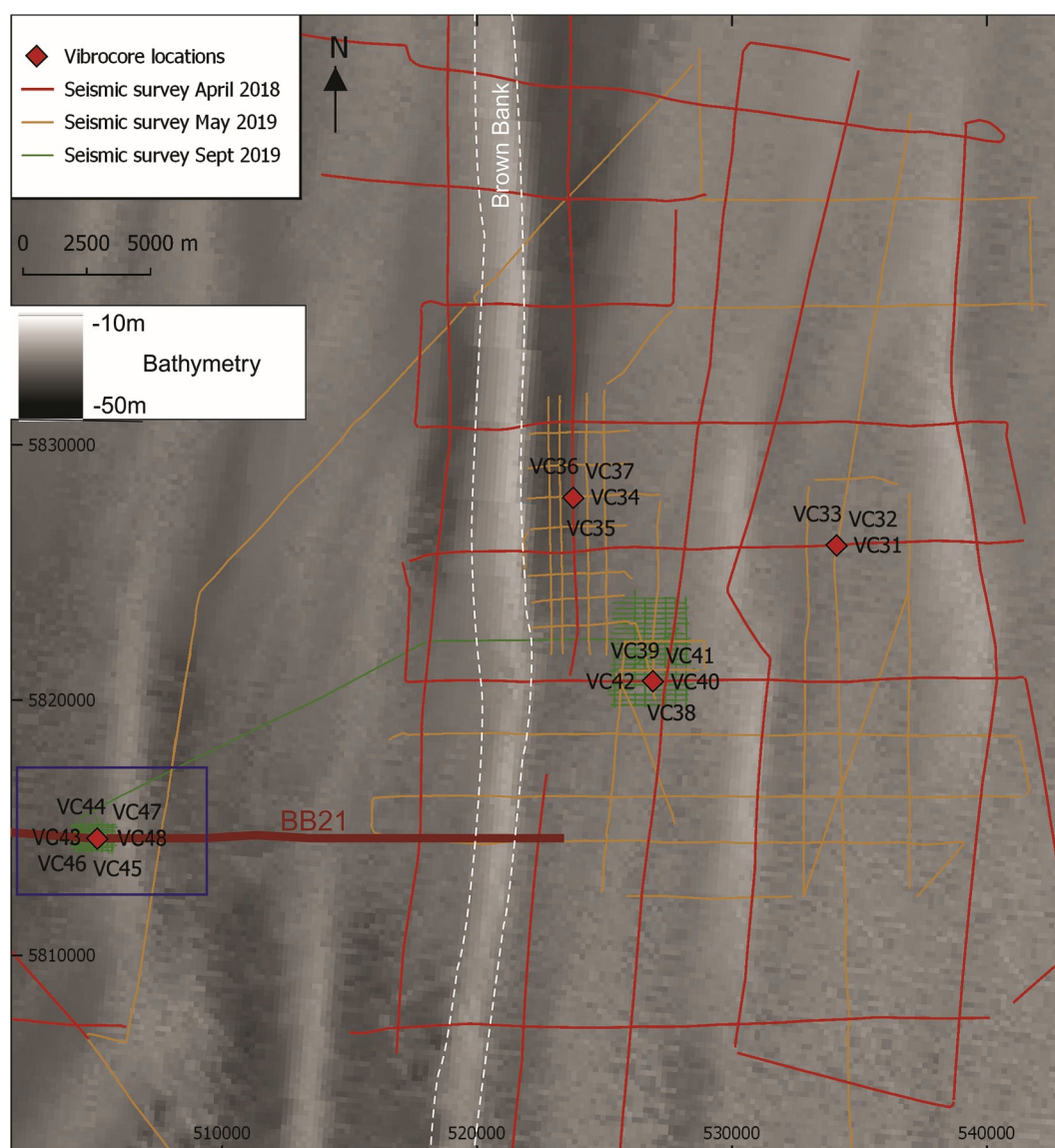
Fig. 2. Map of the seismic surveys and vibrocore sampling undertaken during 2018–2019 by the project team. The blue box indicates the area of interest (site VC43). (For interpretation of the references to colour in this figure legend, the reader is referred to the Web version of this article.)
