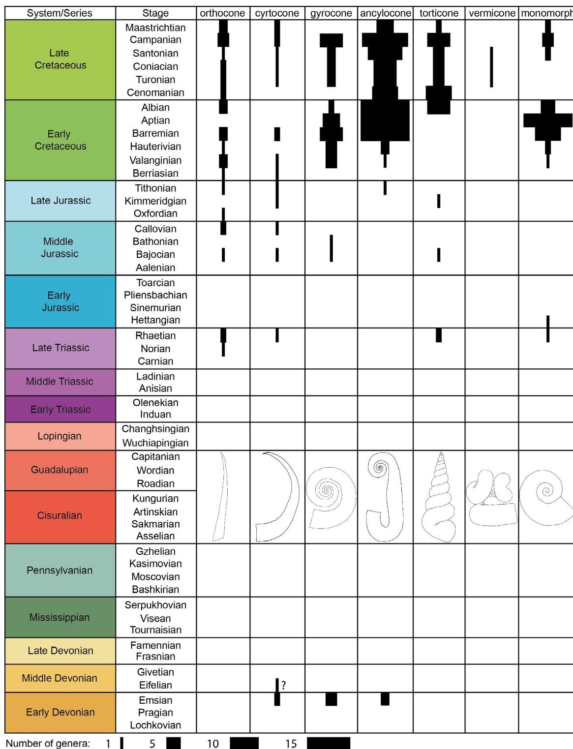
Fig. 11. Stratigraphic distribution of the six arche-morphotypes of heteromorph conchs from the Devonian, Triassic, Jurassic, and Cretaceous. Also shown are secondarily monomorphic forms derived from heteromorphs. After Wright et al. (1996).
