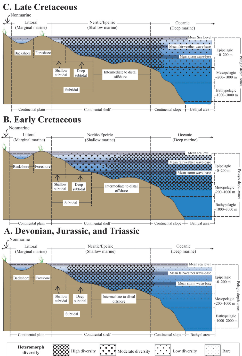
Fig. 8. Heteromorph distributions across marine environments and depth zones during the (A) Devonian, Triassic, and Jurassic, (B) Early Cretaceous, and (C) Late Cretaceous. Based on data from Table S4.
