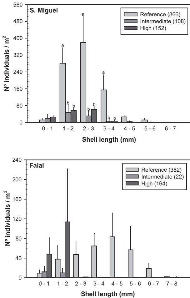
Fig. 3. Abundance (mean ± SE) of the bivalve Ervilia castanea per size-class and CO 2 level in each of the islands; bars with different letters denote significant differences among CO 2 levels within each size class (SNK tests, p < 0.05); values in parenthesis represent mean abundances, across all size classes, at each CO 2 level in each of the islands.
