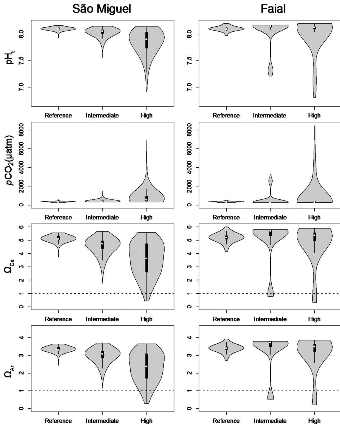
Fig. 2. Violin plots for pH (total scale), \text{CO}_2 partial pressure ( \text{pCO}_2 ), saturation of calcite ( \Omega_{\text{Ca}} ) and aragonite ( \Omega_{\text{Ar}} ); the frequency distribution (grey area), median (white dot) and quartiles (black bars) are presented for each site in each island, across all depths and dates of sampling.
