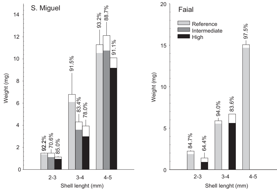
Fig. 4. Individual body weight of the dominant size classes of Evilia castanea per CO 2 level in each Island; dry weight (outline, means \pm SE) and ash weight (filled area, mean); percentage values on top of the bars denote relative ash weight (mean).
