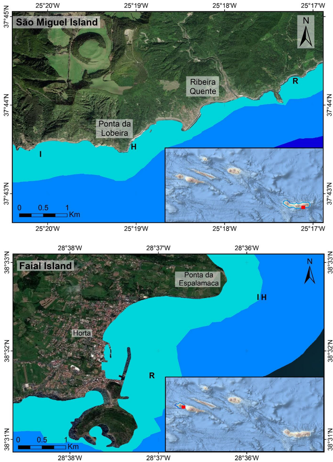
Fig. 1. Map of sampling locations in the central and eastern groups of the Azores archipelago: R - Reference, I - Intermediate CO 2 , H - High CO 2 . The blue gradient represents the 3 depth categories defined for coastal waters around the islands: 0–30 m, 30–200 m and > 200 m.
