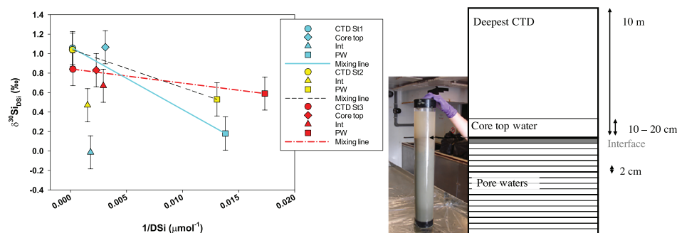
Figure 4. (left) \delta^{30}\text{Si}_{\text{DSi}} against 1/\text{DSi} in \mu\text{mol}^{-1} for deepest CTD (circles), core-top water (diamonds), sediment-water interface (triangle), and porewater at 2 cm depth (square) of Station 1 (blue), Station 2 (yellow), and Station 3 (red). The lines represent the mixing line between the two end-members: deepest CTD and porewater. Conservative mixing is indicated by the samples that fall on the linear mixing curve between the end-members. Loss or gain of Si to or from the porewaters and/or interface waters is indicated by a deviation from linearity. (right) Schematic showing the reservoir depth and scale difference.
