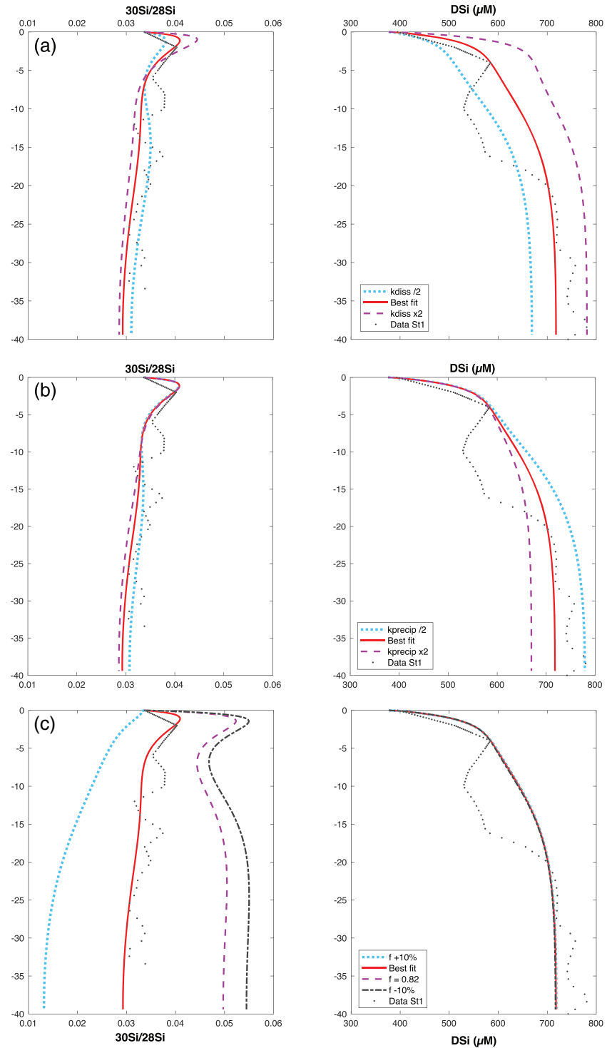
Figure 6. Sensitivity tests of silicic acid (DSi) concentration and ^{30}\text{Si}/^{28}\text{Si} at Station 1, in response to variation of single parameters from the best fit: (a) doubled or halved k_{\text{diss}} BSi rate constant of dissolution, (b) doubled or halved k_{\text{precip}} , molecular coefficient of precipitation, and (c) variation of 10% to DSi consumption in surface water ( f \pm 10\% , where f is the fraction of initial DSi remaining in solution). \delta^{30}\text{Si}_{\text{BSi}} = 0.24\text{‰} corresponds to f = 0.82 (calculated from this study), \delta^{30}\text{Si}_{\text{BSi}} = 0.56\text{‰} corresponds to f - 10\% , \delta^{30}\text{Si}_{\text{BSi}} = -0.65\text{‰} corresponds to f + 10\% . The best fit is achieved with a \delta^{30}\text{Si}_{\text{BSi}} = -0.18\text{‰} . Here, ^{30}\text{Si}/^{28}\text{Si} ratios are equivalent to \delta^{30}\text{Si}_{\text{DSi}} considering that the total abundance of Si isotopes is the sum of ^{28}\text{Si} and ^{30}\text{Si} ; see the SI for a conversion example.
