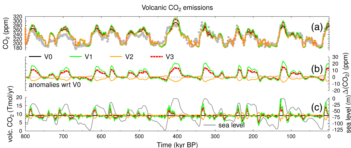
Figure 4. Impact of volcanic \text{CO}_2 outgassing on atmospheric (a, b) \text{CO}_2 . (c) Different volcanic \text{CO}_2 emission scenarios (V0, V1, V2, V3) and sea level, on which they partly depend. V0: volcanic \text{CO}_2 outgassing constant; V1: additional contribution due to the release of land ice masses on the continents (Huybers & Langmuir, 2009); V2: additional contribution due to the release of sea level on mid-ocean ridges and hot spot island volcanoes (Hasenclever et al., 2017); V3: merging effects of V1 and V2. Gray points ( \pm 1\sigma ) in (a) refer to ice core reconstructions (Bereiter et al., 2015). In Subfigure (c) the fluxes are plotted as 1-kyr running mean. Gray line in (c) is the imposed sea level (Bintanja & van de Wal, 2008).
