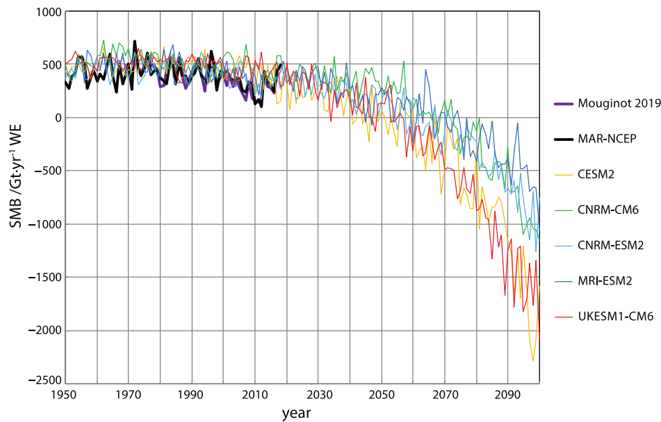
FIGURE 11 Greenland Ice Sheet annual SMB after Mouginito et al. (2019) (purple line), based on the RACMO regional climate/SMB model, and as simulated by MAR using NCEP-NCAR v1 Reanalysis data from 1950–2018 (black line) and MAR runs using five different CMIP6 GCMs (MAR-CESM2, MAR-CNRM-CMIP6, MAR-CNRM-ESM2, MAR-MRI-ESM2, MAR-UKESM1-CMIP6) and the SSP5-8.5 scenario as forcing (other colour lines) (Hofer et al. , in review). Note this does not include topographic changes or surface-elevation feedbacks, which would likely increase the changes shown here, especially after 2070
