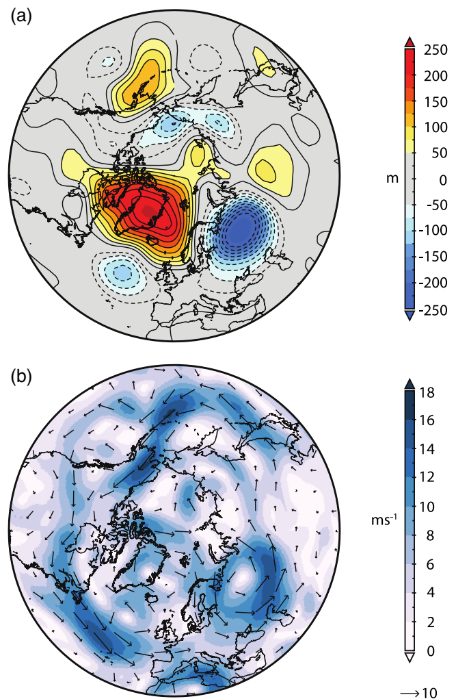
FIGURE 9 NCEP/NCAR Reanalysis v1 mean (a) 500 hPa geopotential anomalies and (b) 700 hPa vector winds indicating direction of anomalous south-easterly airflow over Greenland during the high Greenland Blocking (GB) and high ice-melt episode from 30 July to August 4, 2019, during which consecutive daily GB anomalies were all >2\sigma . For panel (a) negative contours are dotted and the zero contour is omitted
