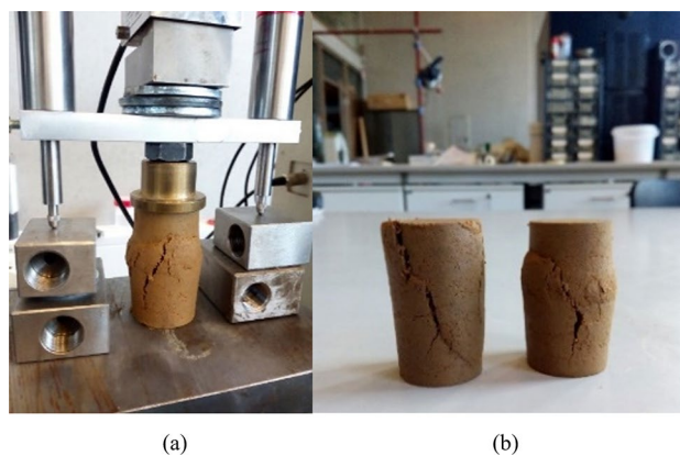
Fig. 8 Simple compression test: a sample during test, b sample after test
