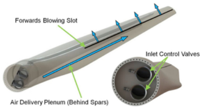
Fig. 6. Circulation control system. Courtesy of Kohana Technologies Inc.
