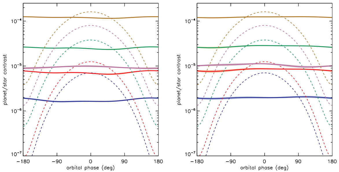
Fig. B.24. Emission phase curves computed for an aquaplanet with a 1 bar CO 2 -dominated atmosphere in synchronous rotation ( left ) and 3:2 spin-orbit resonance ( right ).
