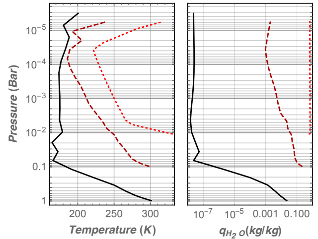
Fig. 7. Annual mean atmospheric temperature ( left ) and water vapor ( right ) vertical profiles of atmospheres with different total surface pressure (solid black: 1 bar; dashed, dark red: 0.1 bar; dotted red: 0.01 bar). The composition of all three atmospheres is N 2 with 376 ppm of CO 2 and a variable amount of water vapor. The profiles are shown at the substellar point, but horizontal variations are fairly small above the 0.1 mbar level due to an efficient transport. Decreasing the surface pressure increases the water vapor ratio in the upper atmosphere drastically.
