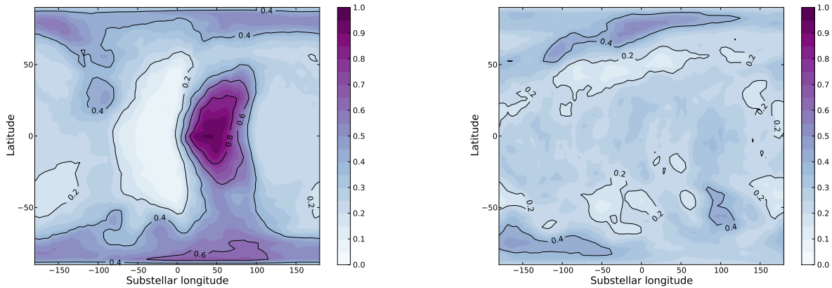
Fig. B.2. Cloud maps for an aquaplanet with a 1 bar CO_2 atmosphere. Left : synchronous rotation. Right : 3:2 spin-orbit resonance. In both cases, longitude is given relative to the substellar point. Colors indicate the fractional cloud cover, averaged over 2 orbits.
