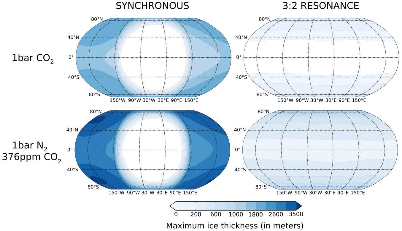
Fig. 4. Maximum ice thickness calculated from 4 completely dry GCM simulations made of 2 different atmospheric compositions (1 bar pure CO 2 atmosphere, 1 bar N 2 -dominated atmosphere with 376 ppm of CO 2 ) and 2 orbital configurations (synchronous and 3:2 resonance). The maximum ice thickness is calculated from the basal melting condition derived from the mean surface temperature from Fig. 3. The internal heat flux is assumed to be 110 mW m -2 for the synchronous orbit cases and 180 mW m -2 for the asynchronous cases. The global equivalent thickness of ice is 940 m (1 bar of CO 2 ) and 1650 m (Earth atmosphere) for the synchronous rotation, and 115 m and 490 m for the 3:2 resonance, respectively. The amount of ice calculated from the 1 bar CO 2 simulation is probably a lower estimate since CO 2 would collapse, making the cold points even colder.
