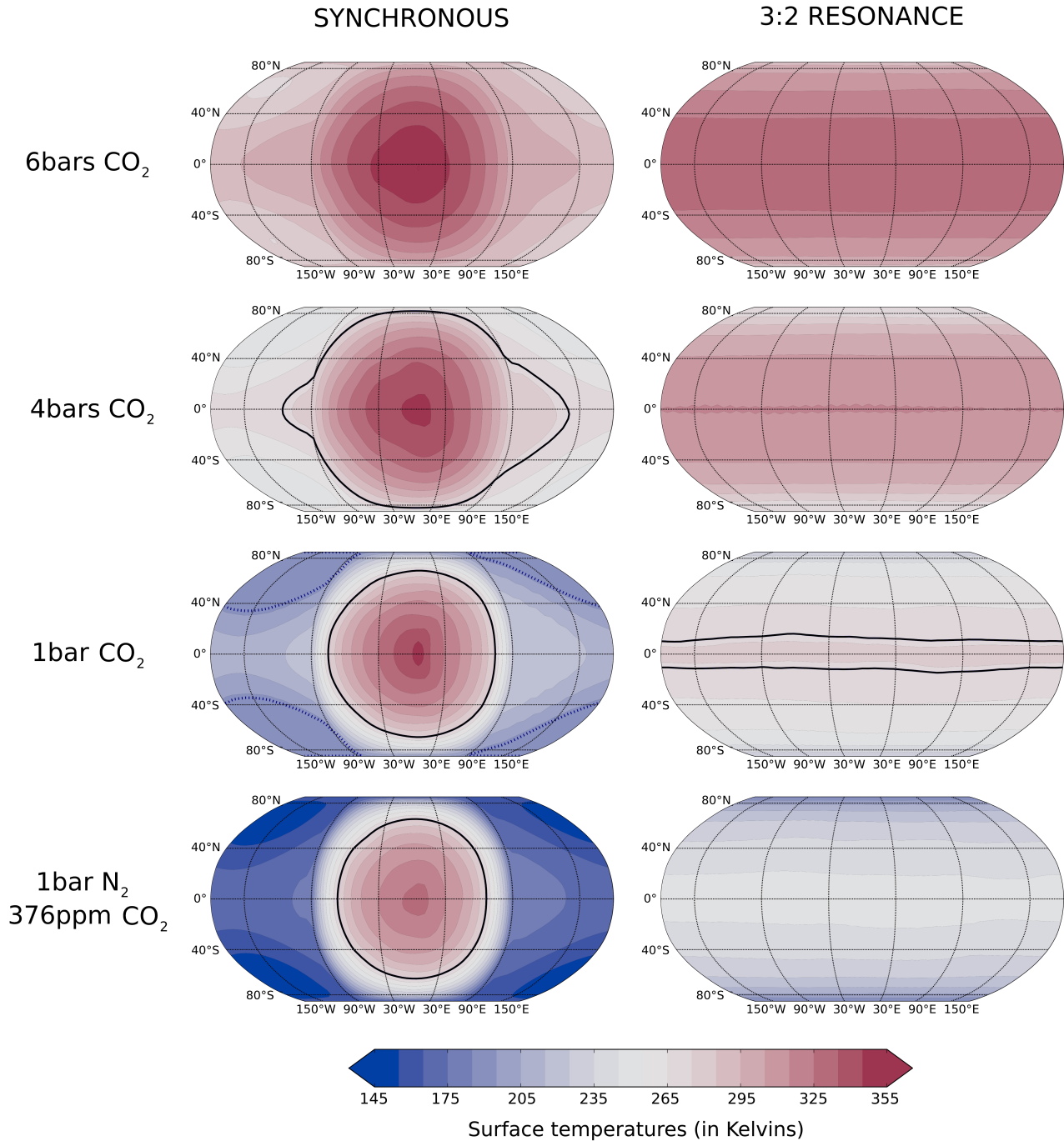
Fig. 3. Biennial mean surface temperatures of completely dry atmospheres, for 2 orbital configurations (synchronous and 3:2 orbital resonance) and 4 atmospheric compositions and pressures (6 bars of pure CO 2 , 4 bars of pure CO 2 , 1 bar of pure CO 2 and 1 bar of N 2 + 376 ppm of CO 2 – Earth-like atmosphere). The solid black line contour corresponds to the 273.15 K isotherm; the dashed blue line contour indicates the regions where the atmospheric CO 2 collapses permanently into CO 2 ice deposits. The 1 bar pure CO 2 (synchronous) simulation is not stable in the long term since CO 2 would collapse at the two cold points.
