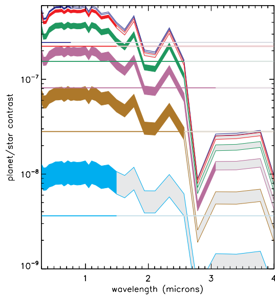
Fig. B.8. Reflection spectra computed for a dry planet with a Venus-like atmosphere (including aerosols).
