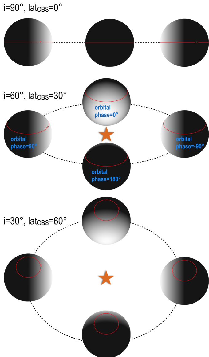
Fig. 11. Phase curves and observing geometries. We computed reflected and emitted light curves for 3 inclinations as follows: 90, 60, and 30^\circ corresponding to subobserver latitude of 0, 30, and 60^\circ , respectively (as the we assumed a null obliquity). The subobserver latitude is indicated with a red line. In Appendix B, phase curves are shown only for an inclination of 60^\circ (the median value for randomly oriented orbits).
