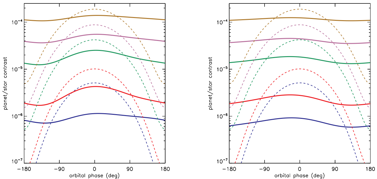
Fig. B.22. Emission phase curves computed for an aquaplanet with a 10 mbar \text{N}_2 -dominated (+376 ppm of \text{CO}_2 ) atmosphere in synchronous rotation ( left ) and 3:2 spin-orbit resonance ( right ).
