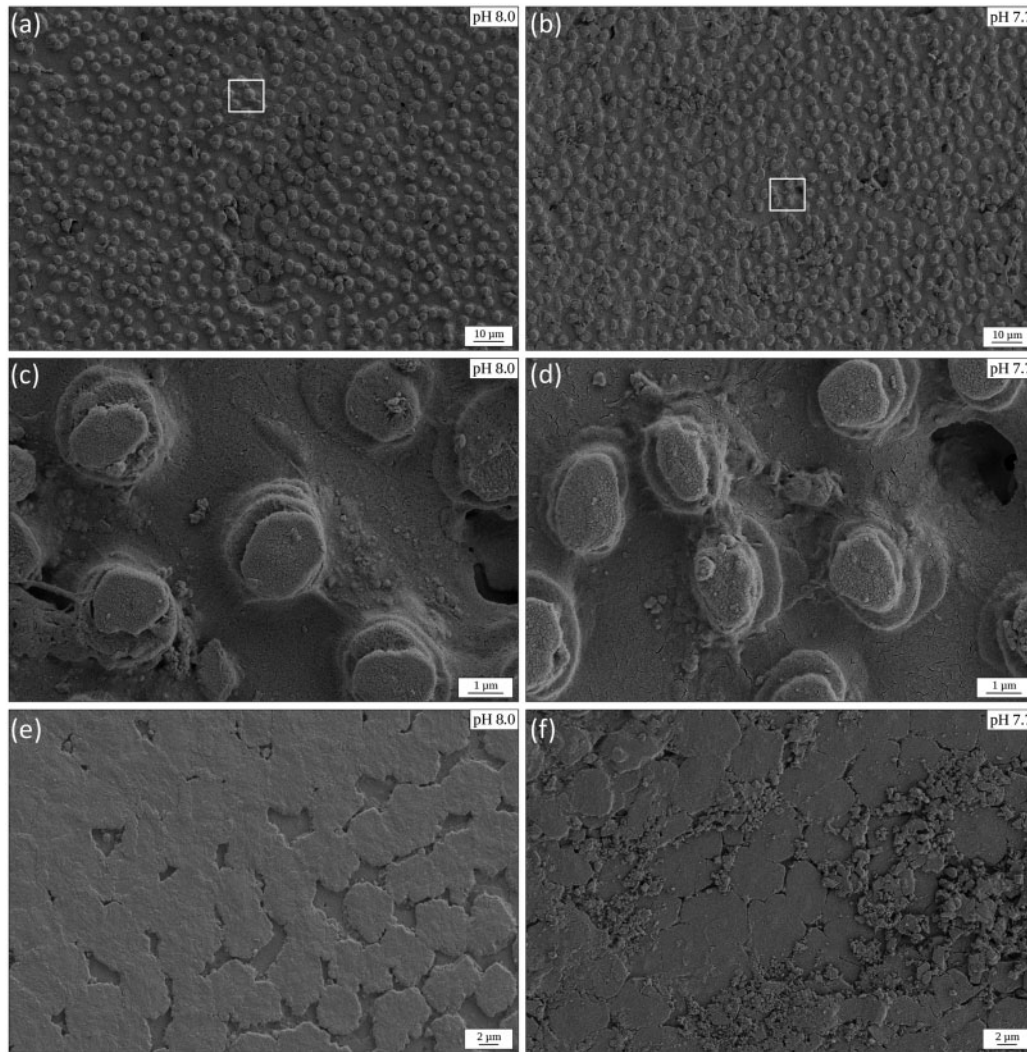
Figure 7. SEM images of the inner nacreous layer in control abalone shell (pH 8.0, a, c, e) and in abalone exposed to pH 7.7 for 4 months (b, d, f). (a and b) Inner nacreous layer showing a homogenous surface with growing aragonite platelets. (c and d) Magnification of the nacre growth region, boxed in (a) and (b), respectively. (e and f) Detail of the transition region between immature and mature nacre showing dissolution of the aragonite platelets under lower pH (f).
