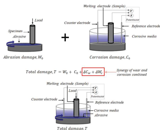
Figure 1 Schematic representation of synergy in the novel abrasion-corrosion test rig.
