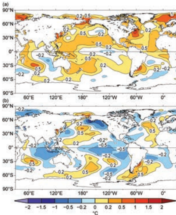
FIG. 3.1. (a) Annually averaged ERSSTv5 SSTA ( ^{\circ}\text{C} ) for 2017 relative to a 1981–2010 climatology and (b) difference of annually averaged SSTAs between 2017 and 2016 (2017–2016).
