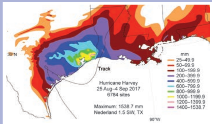
FIG. SB4.5. Observed rainfall totals in association with Harvey and its remnants. (Source: Weather Prediction Center, NOAA.)
