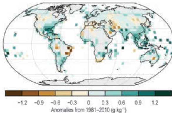
(n) Surface Specific Humidity
