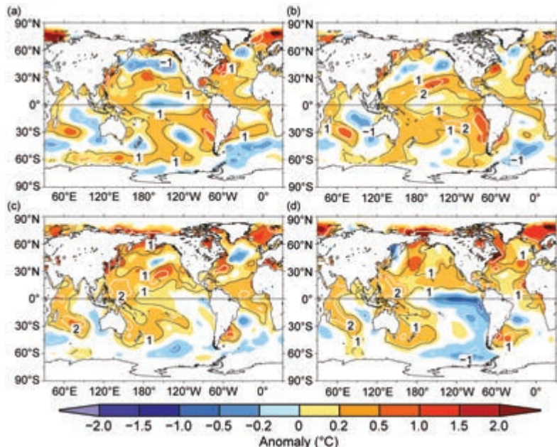
FIG. 3.2. Seasonally averaged SSTAs of ERSSTv5 ( ^{\circ}\text{C} ; colors) for (a) Dec 2016–Feb 2017, (b) Mar–May 2017, (c) Jun–Aug 2017, and (d) Sep–Nov 2017. Normalized seasonal mean SSTA based on seasonal mean std. dev. for 1981–2010 are indicated by contours of -1 (dashed white), +1 (solid black), and +2 (solid white).
