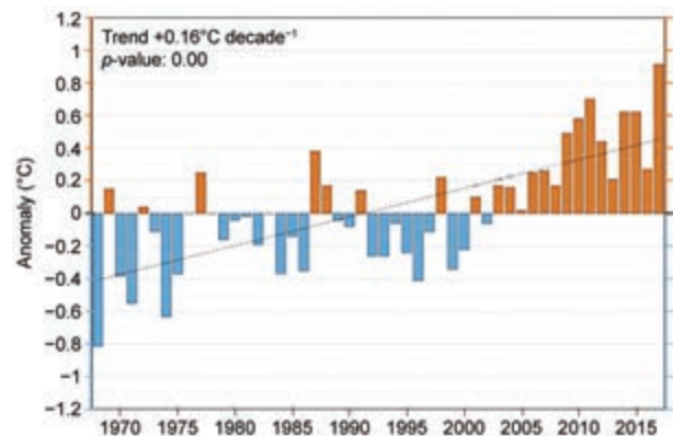
FIG. 7.30. Annual mean temperature anomalies (°C; 1981–2010 base period) for Réunion Island, 1968–2017. (Source: Météo-France.)
