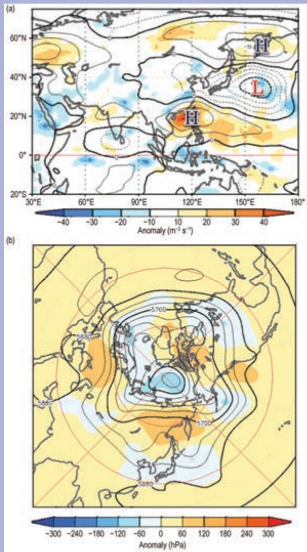
FIG. SB7.5. (a) Stream function anomalies at 850-hPa (contours) and OLR anomalies ( m^2 s^{-1} ; color shadings) averaged over 1–20 Aug 2017. Thick and thin contours are intervals of 10 \times 10^6 and 2.5 \times 10^6 m^2 s^{-1} , respectively. For the NH, solid and dashed lines indicate anticyclonic and cyclonic circulation anomalies, respectively. For the SH, vice versa. (b) 500-hPa height anomaly in the NH averaged over 1–20 Aug 2017. Contours show 500-hPa height at intervals of 60 m. Shading indicates anomalies. Base period is 1981–2010.
