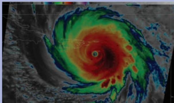
FIG. SB7.1. Satellite image of the center of Hurricane María located southeast of St. Croix, USVI on 20 September 2017. (Source: NOAA/NWS.)
