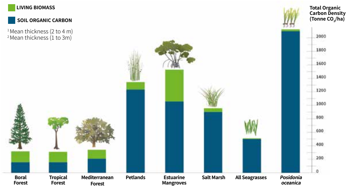
Figure 5: Comparison of soil C_{org} storage in the top metre of the soil with total ecosystem C_{org} storage for major ecosystem types. Here, the seagrass Posidonia oceanica is a unique seagrass in terms of the quantity of organic carbon that can be stored in its sediments and matte. Soil Data: Top meter sediment [12, 111, 112, 113].
