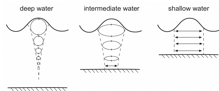
Figure 4.5. Motion of water particles under surface gravity waves at different water depths (Masselink et al., 2011).
