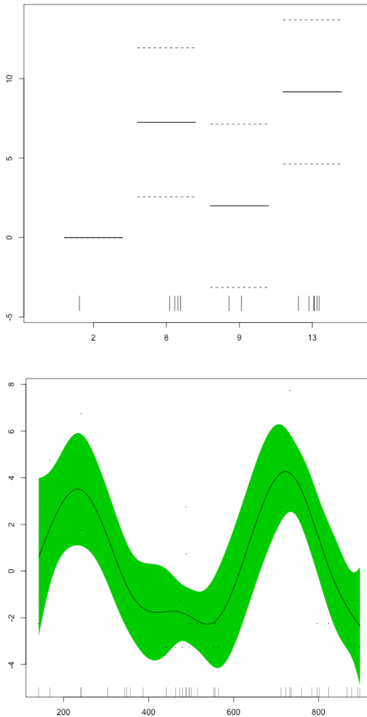
Figure 5.7. Rijkswaterstaat seagrass surveys (SGS). Left panel: factors for best fits for univariate data model describing the relationship between a relative index for seagrass occurrence (y-axis) and measurement section (x-axis) in mm for SGS 2006-2009. Right panel: smoother for best fit for univariate data model describing the relationship between a relative index for seagrass occurrence (y-axis) and sediment height (x-axis) in mm for SGS 2010-2017 (see Table 5.6 for statistics).
