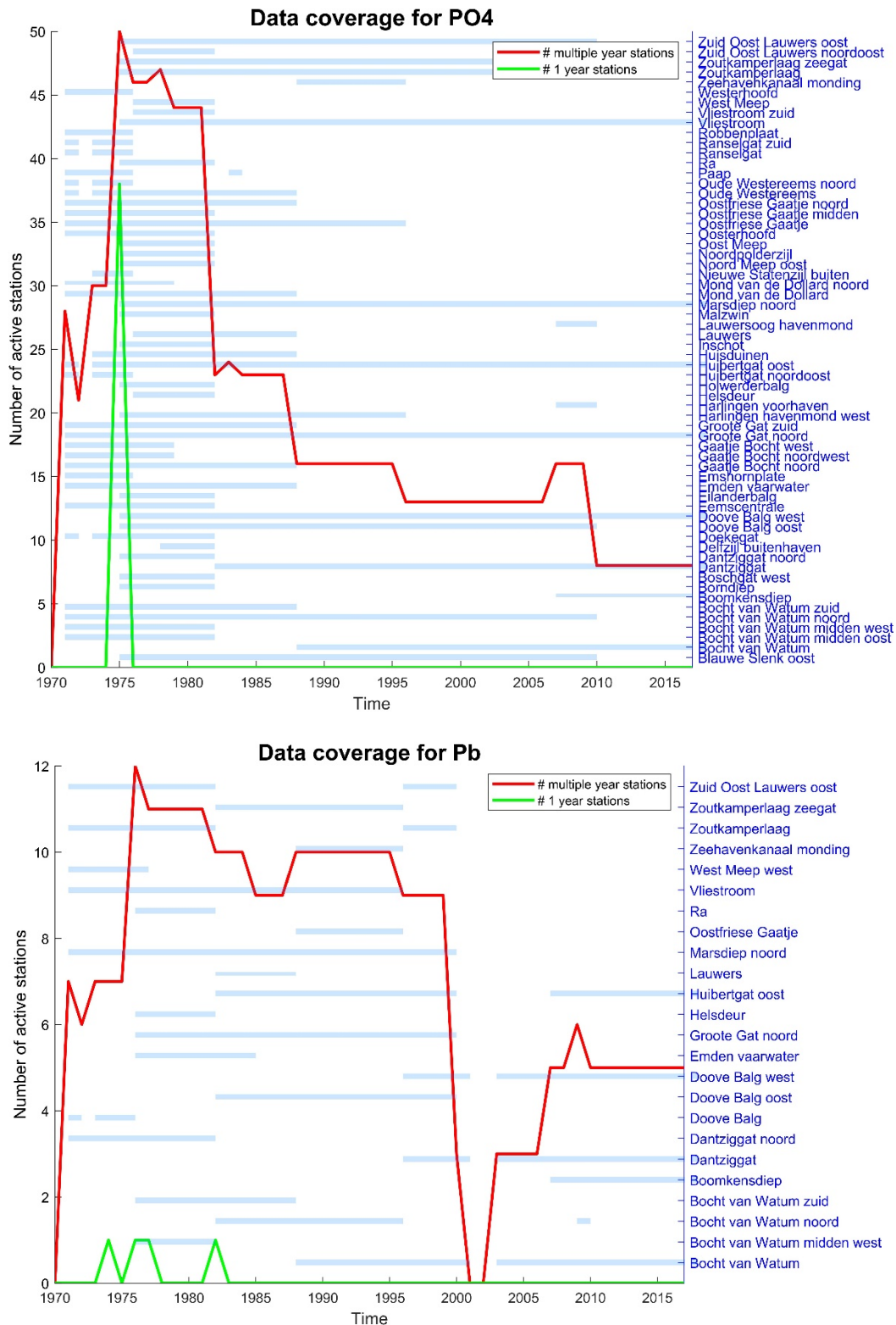
Figure 3.1. Active Rijkswaterstaat monitoring stations monitoring ortho-phosphate (above, PO 4 ) and lead (below, Pb) from 1970 to 2017.
