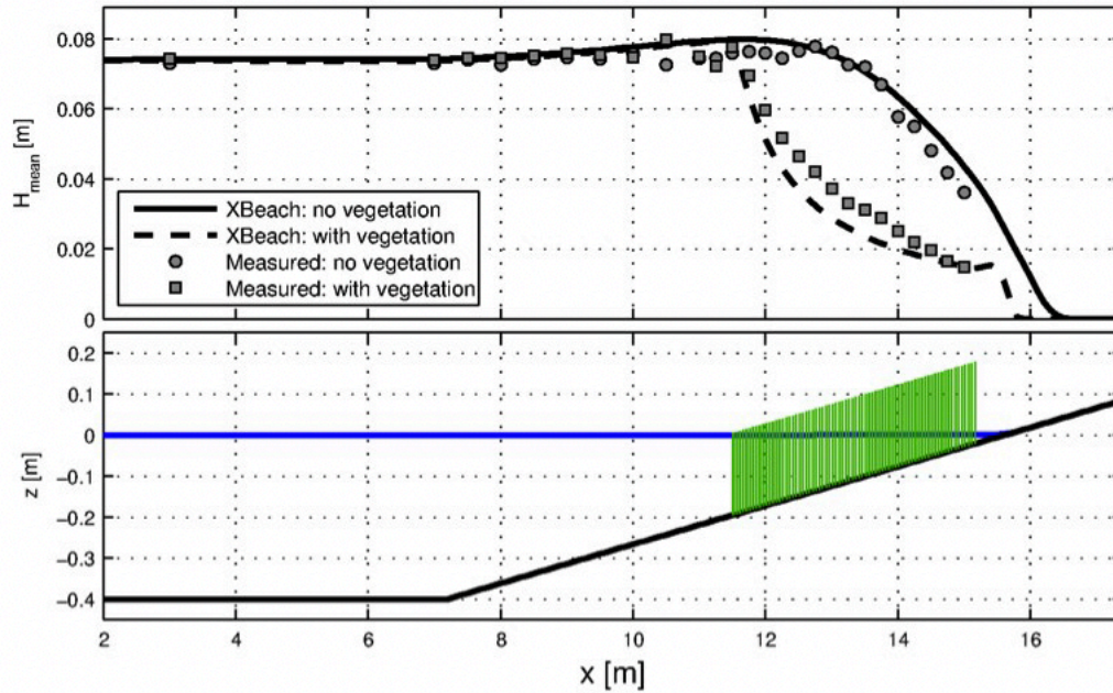
Figure 4.6. Top panel shows the predicted (straight and dotted line, based upon XBeach model) and observations (circles and squares) effects of vegetation on the significant wave height ( H_{mean} ; m) based upon a sediment profile (height z in m, transect x in m) and height of the vegetation when present (green) as depicted in the bottom panel (Deltares, 2014).
