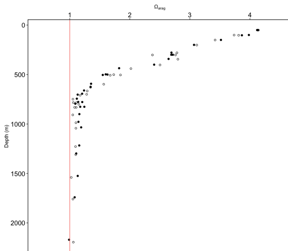
Supplementary Figure A1. Aragonite saturation state profiles for the Anegada Passage using measured (closed circle) and model predicted (open circle) \Omega_{arag} values. A solid red vertical line at \Omega_{arag} = 1 represents the aragonite saturation horizon.
