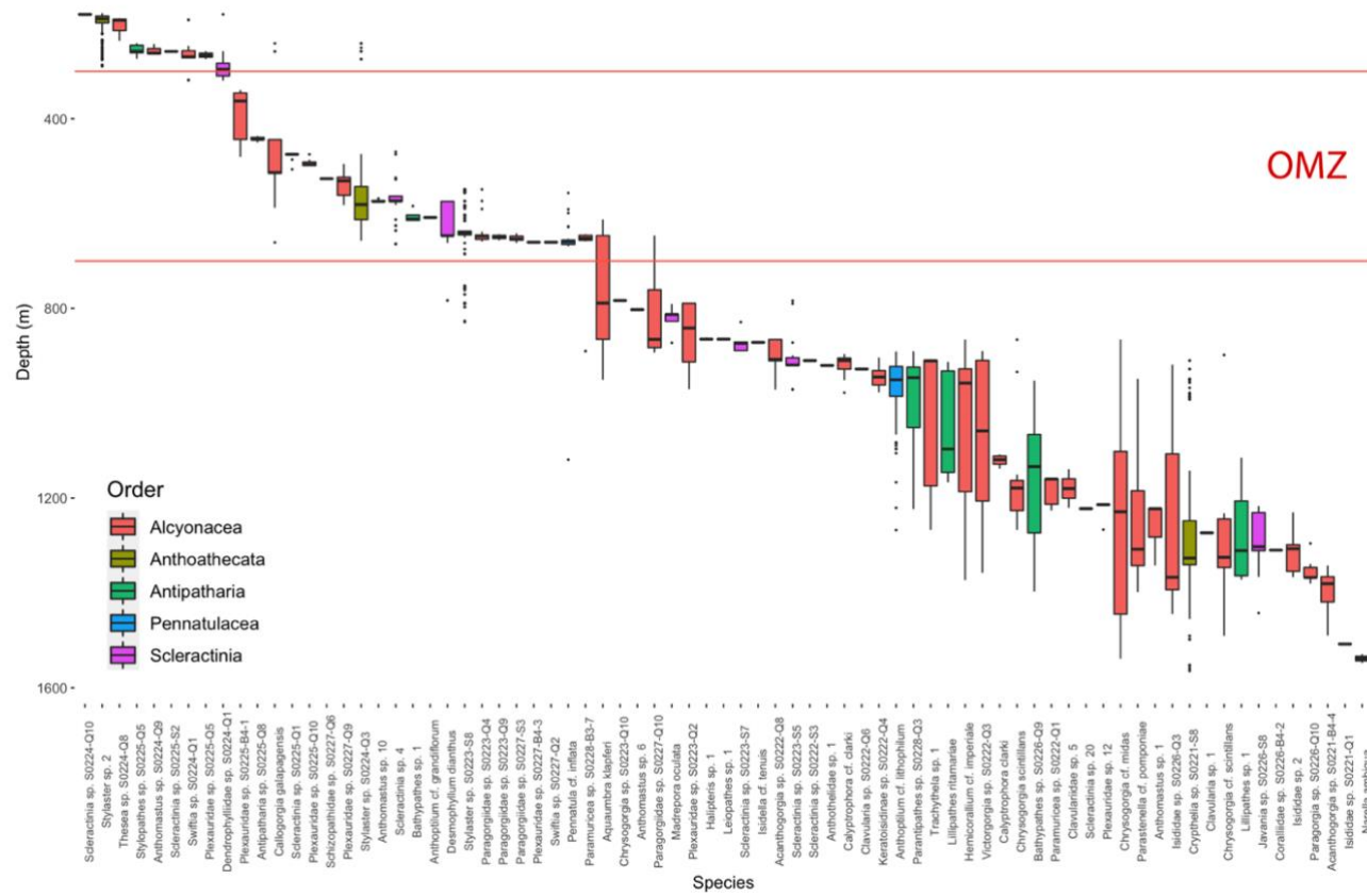
Figure 4.3 Boxplot of species distribution across depth. Species are arranged left to right by increasing median depth of distribution. Boxes are colored by taxonomic order for each species. OMZ depths (300-700 m) are indicated by solid red lines and bold red text.
