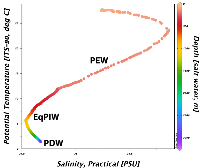
Figure 3.3 Temperature-salinity diagram from the sea surface to 3000 m collected via CTD rosette downcast North of Kanton Atoll. The approximate depth of each water mass identified below 200 m is overlaid in bold. Plot was constructed using Ocean Data View v5.1 (Schlitzer, 2019).
