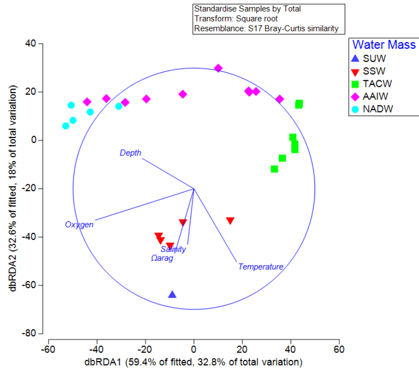
Figure 2.7 Distance-based linear model and redundancy analysis of coral assemblages and oceanographic variables. Sample points represent one 100 m depth assemblage. Axes shown are the results of a distance-based redundancy analysis with percent variation explained by the first and second axes.
