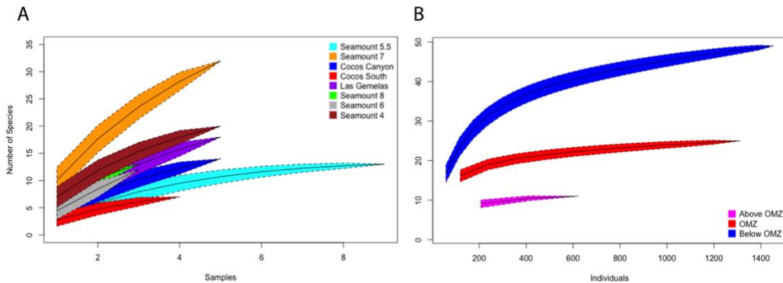
Figure 4.4 Species accumulation and rarefaction analyses. Permuted (1000 permutations) species accumulation (Coleman et al., 1982) curves are assessed between sites (A). Sample-based rarefaction curves (B) are indicated for each layer of the water column corresponding to depths above (100-300 m), below (700-1600 m), and within (300-700 m) the oxygen minimum zone. For both plots, confidence intervals (95%) are indicated by polygons around curve bounded by dashed lines.
