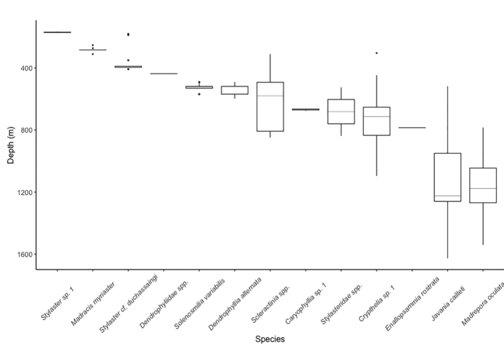
Figure 2.3 Depth distribution for scleractinian and stylasterid corals occurring on Dog, Conrad, and Noroît Seamounts. Box plots represent the interquartile range with whiskers extending from the upper and lower quartiles to the minimum and maximum values. Horizontal lines represent the median depth. Individual points represent outliers. Species are arranged on the x-axis from shallowest to deepest by median depth of occurrence.
