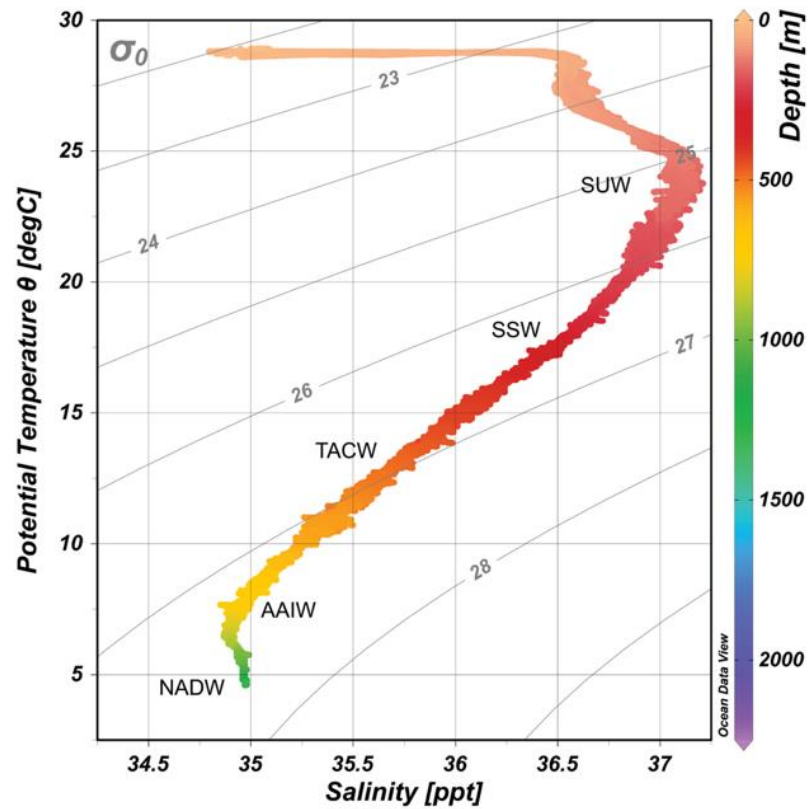
Figure 2.2 Temperature-salinity plot for the Anegada Passage based on CTD water column profiles. Water masses are overlaid and abbreviated by the following: SUW=Subtropical underwater, SSW=Sargasso Sea Water, TACW= Tropical Atlantic Central Water, AAIW=Antarctic Intermediate Water, and NADW=North Atlantic Deep Water. Isopycnal surfaces ( \sigma_\theta ) are indicated in gray.
