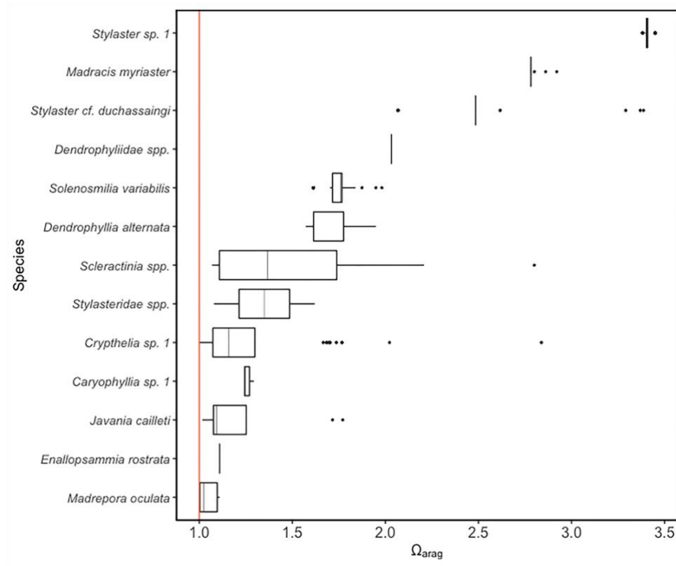
Figure 2.4 Distribution of scleractinian and stylasterid species against model predicted \Omega_{\text{Arag}} values on the Anegada Passage seamounts. Box plots represent the interquartile range with whiskers extending from the upper and lower quartiles to the minimum and maximum values. Vertical lines represent the median aragonite saturation state. Individual points represent outliers. Species are arranged on the y-axis from highest to lowest median aragonite saturation occurrence. A solid red vertical line indicates the aragonite saturation horizon, where \Omega_{\text{Arag}}=1 .
