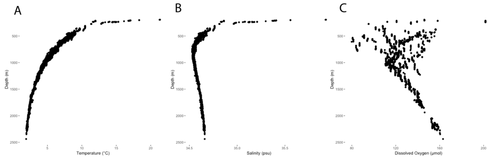
Figure 3.4 Temperature (A), salinity (B), and dissolved oxygen (C) profiles from ROV CTD unit records co-occurring with deep-water coral observations between 193 and 2439 m.
