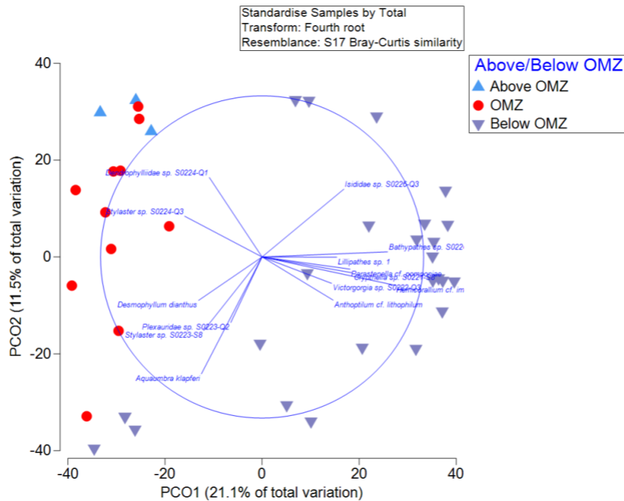
Figure 4.9 Principle coordinates analysis of 39 samples designated as above, below or within the OMZ. A circle with vector lines indicates any correlations ( R = > 0.40 cutoff) of species with samples in the PCO space.
