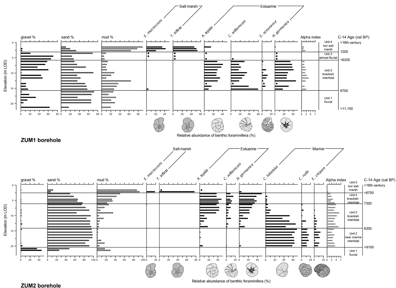
Fig. 3. Vertical distribution of grain size (%), relative abundance of main foraminiferal species (%), alpha diversity index, depositional environment and C-14 age (median values of calibrated radiocarbon dates) with depth (m) in boreholes ZUM1 and ZUM2, Urola estuary (Basque Coast Geopark). Black dots indicate presence of the species in assemblages with less than 100 foraminiferal tests.
