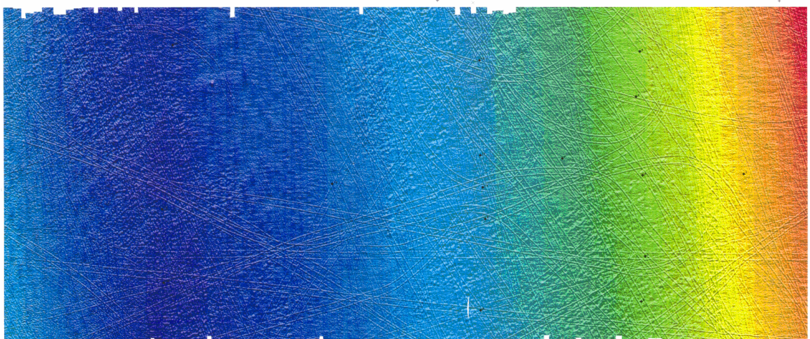
Figure 3.4 Multibeam sonar image of the transition of the lower shoreface to the inner continental shelf. The area is located 5-10 km offshore Noordwijk aan Zee, in water depths of 15 m (red colour) to 20 m (dark blue colour). Landward is to the right. The area is dominated by a flat seafloor (slope less than 1:1000) without major bedforms. Megaripples and tracks made by beam-trawling fishermen are found at the surface.
