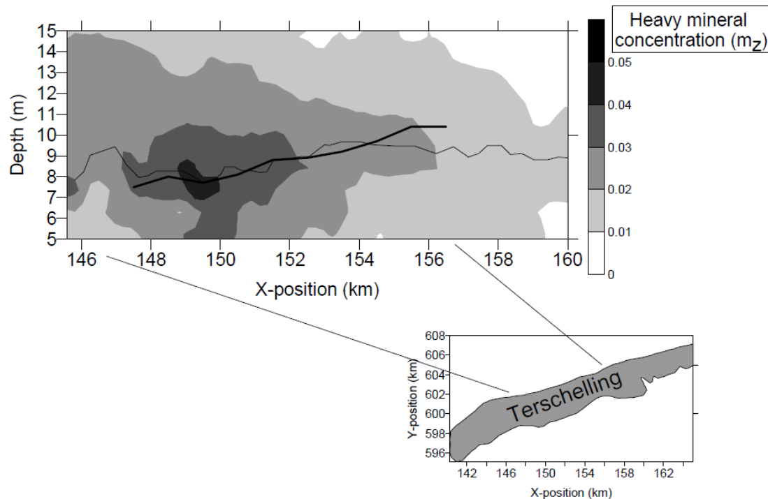
Figure 2.7 Longshore variation of the heavy-mineral concentration as function of water depth at Terschelling. The thin line represents cross-shore maxima in the heavy-mineral concentration. The thick line shows the variation of the 25-years depth of closure determined from profile measurements by Marsh et al. (1998). Figure taken from Koomans (2000).
