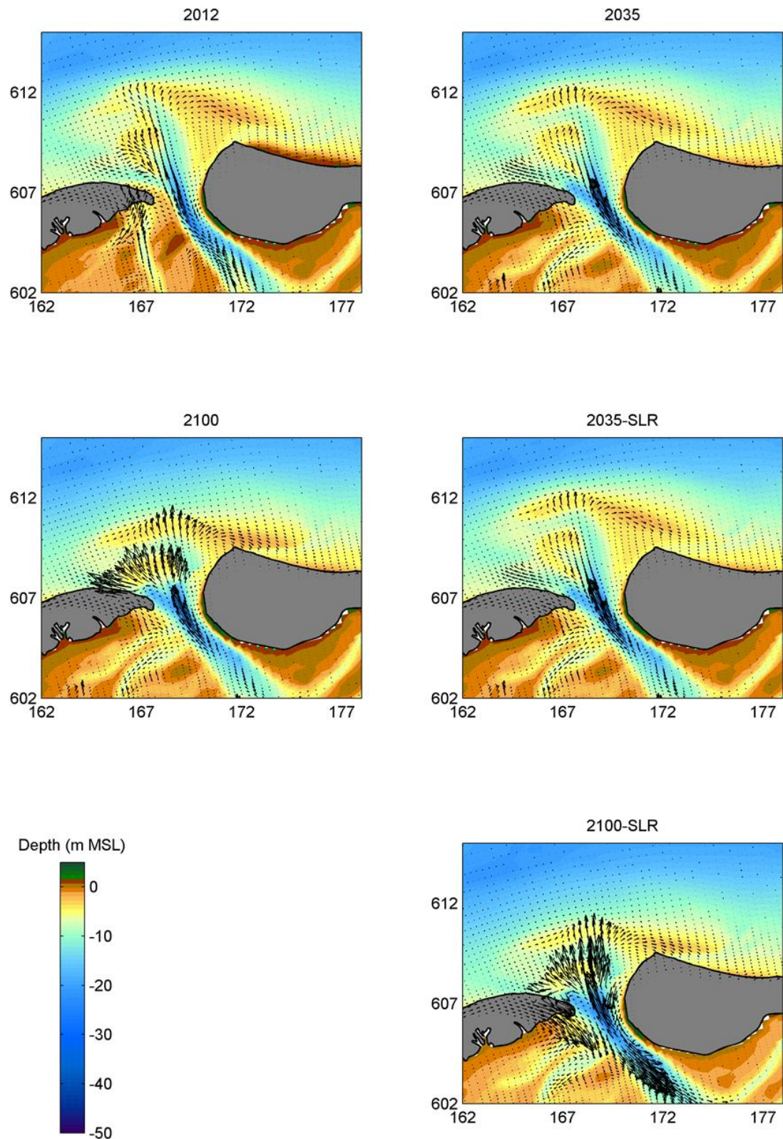
Figure 5.19 Computed transport vectors in the Ameland Inlet for the present situation, 2035 and 2100
