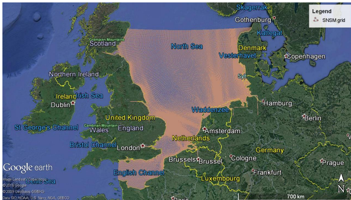
Figure 5.9 Southern North Sea Model grid
