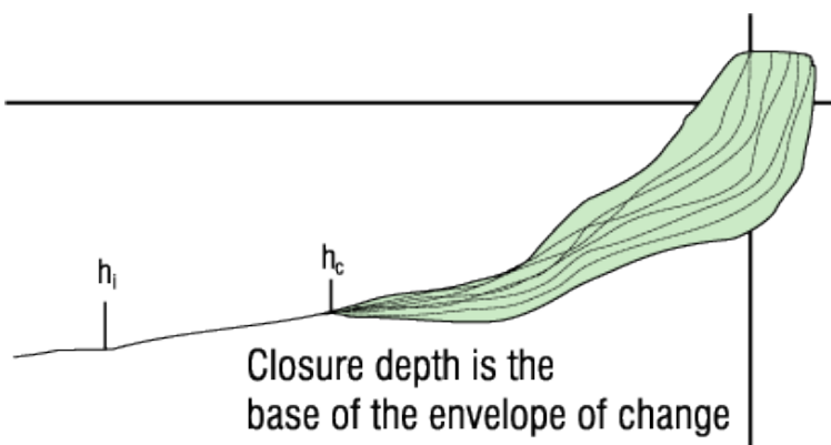
Figure 2.4 Illustration of the morphological envelope in order to define the closure depth.
