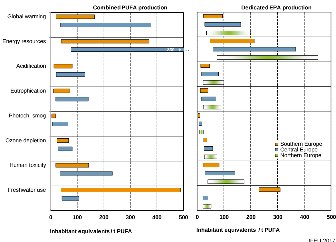
Fig. 4-3 Ranges of results for analysed scenarios of PUFA production. Results are expressed in inhabitant equivalents (IE) 9 . Avoided impacts due to the use of co-products were credited.
